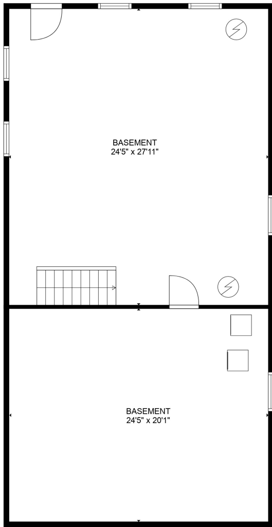
FLOOR 1
