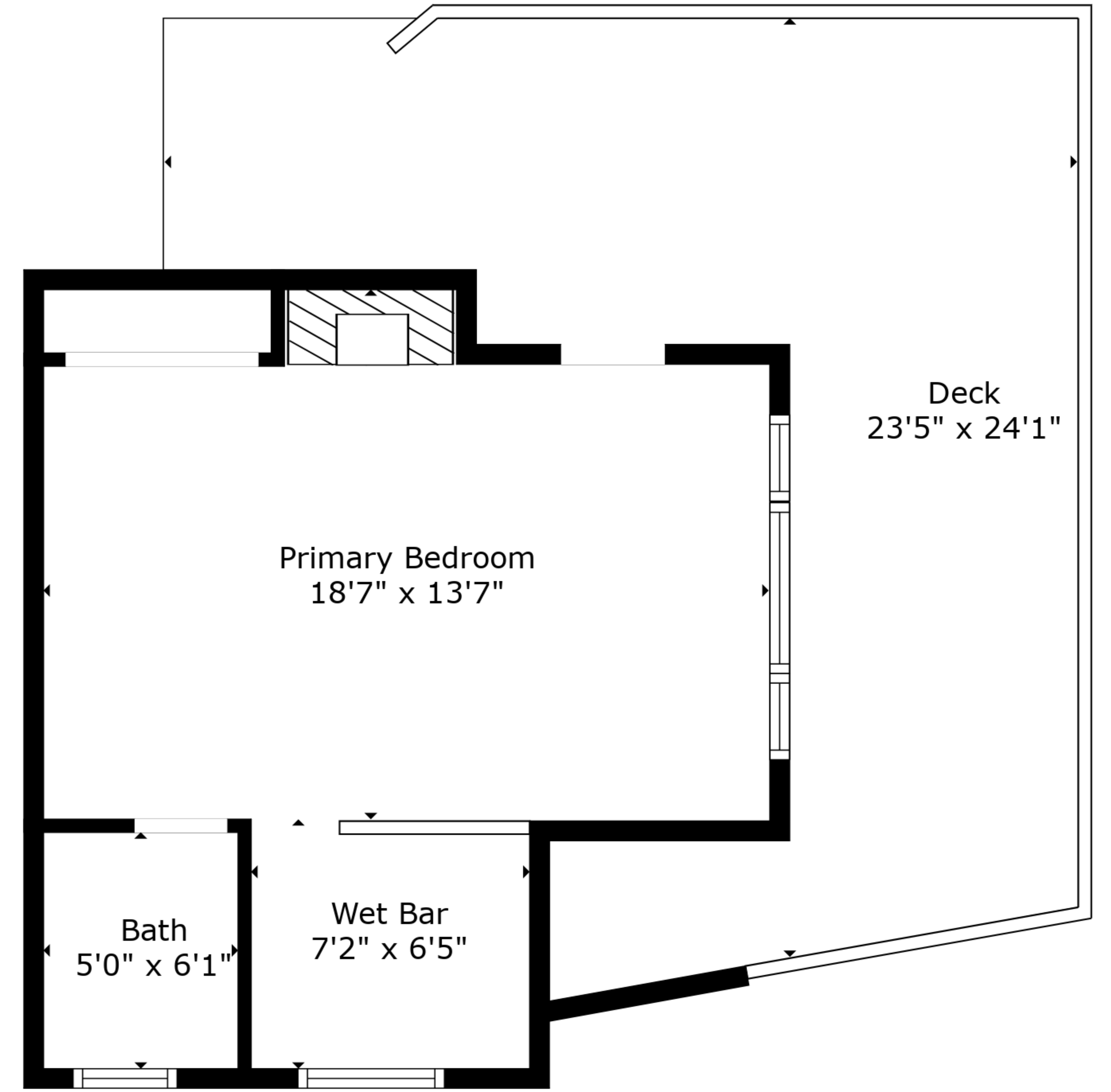
Floor 3
