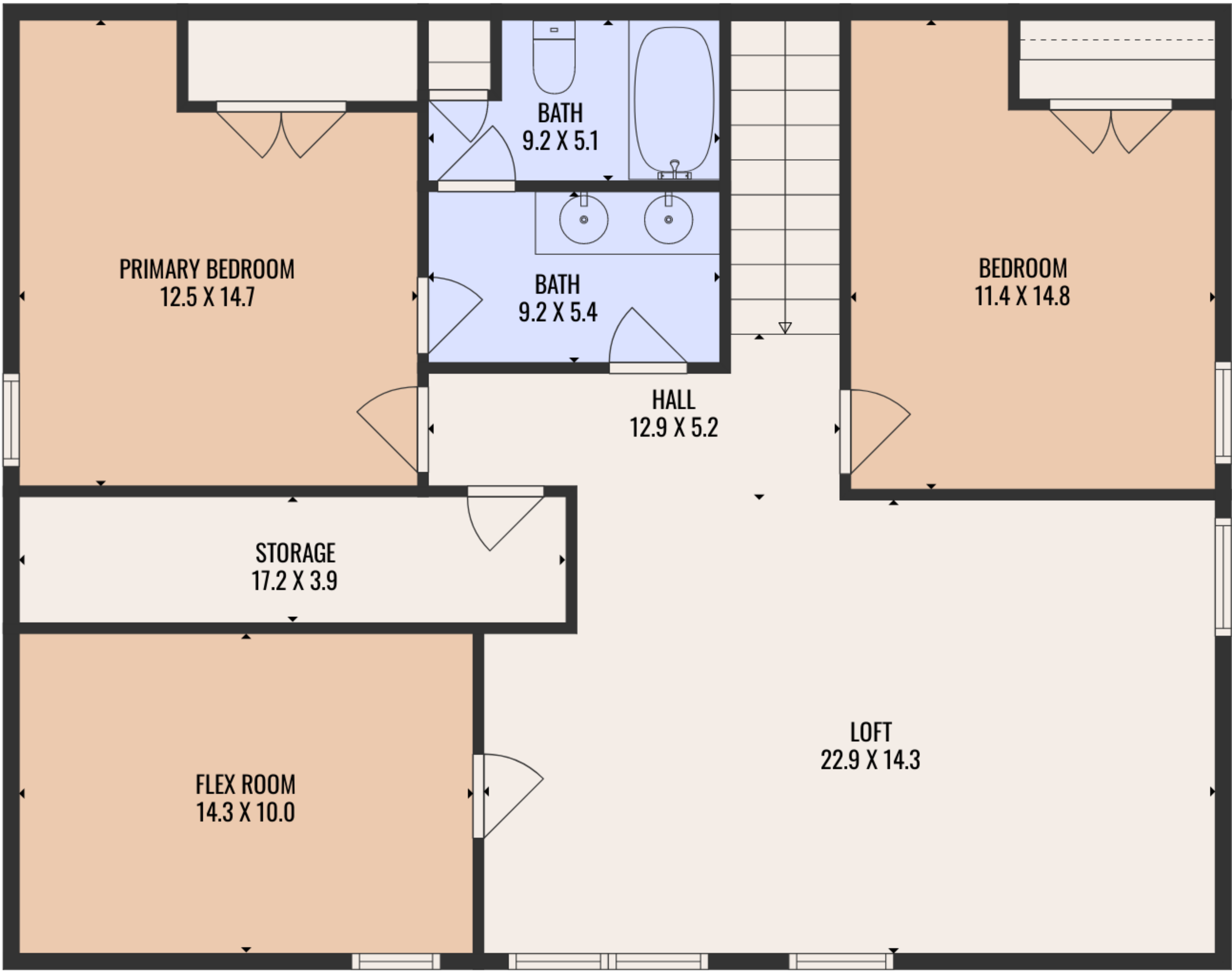
FLOOR 2
