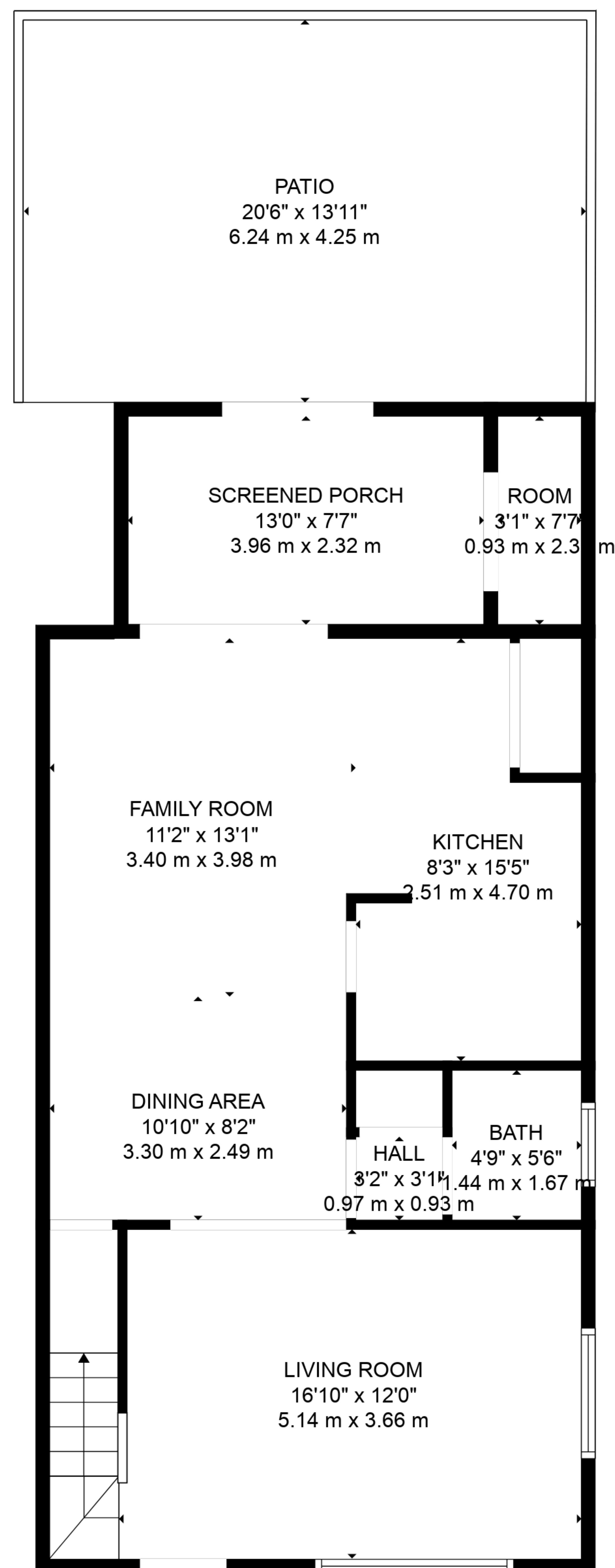
FLOOR 1
