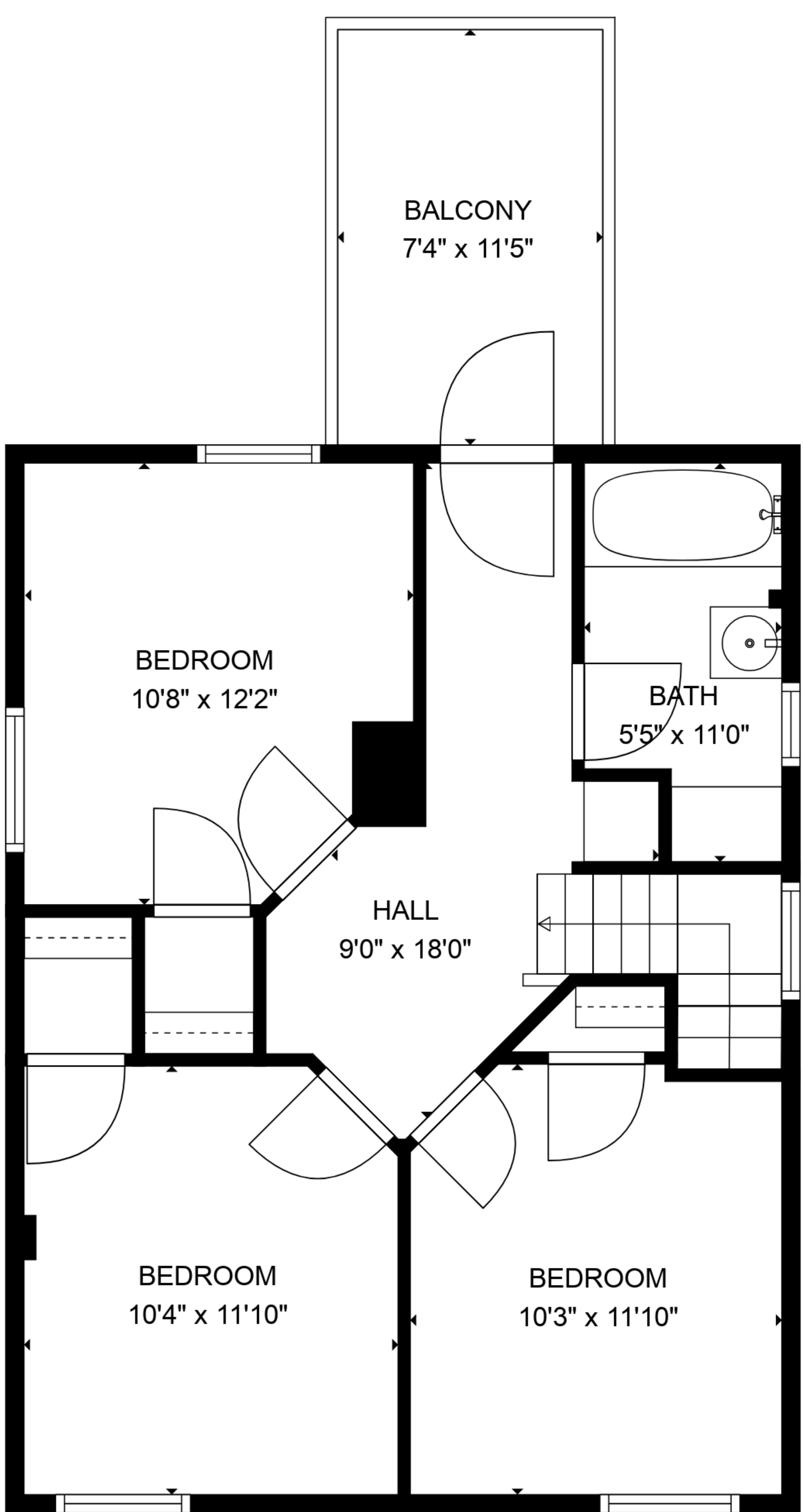
FLOOR 3
