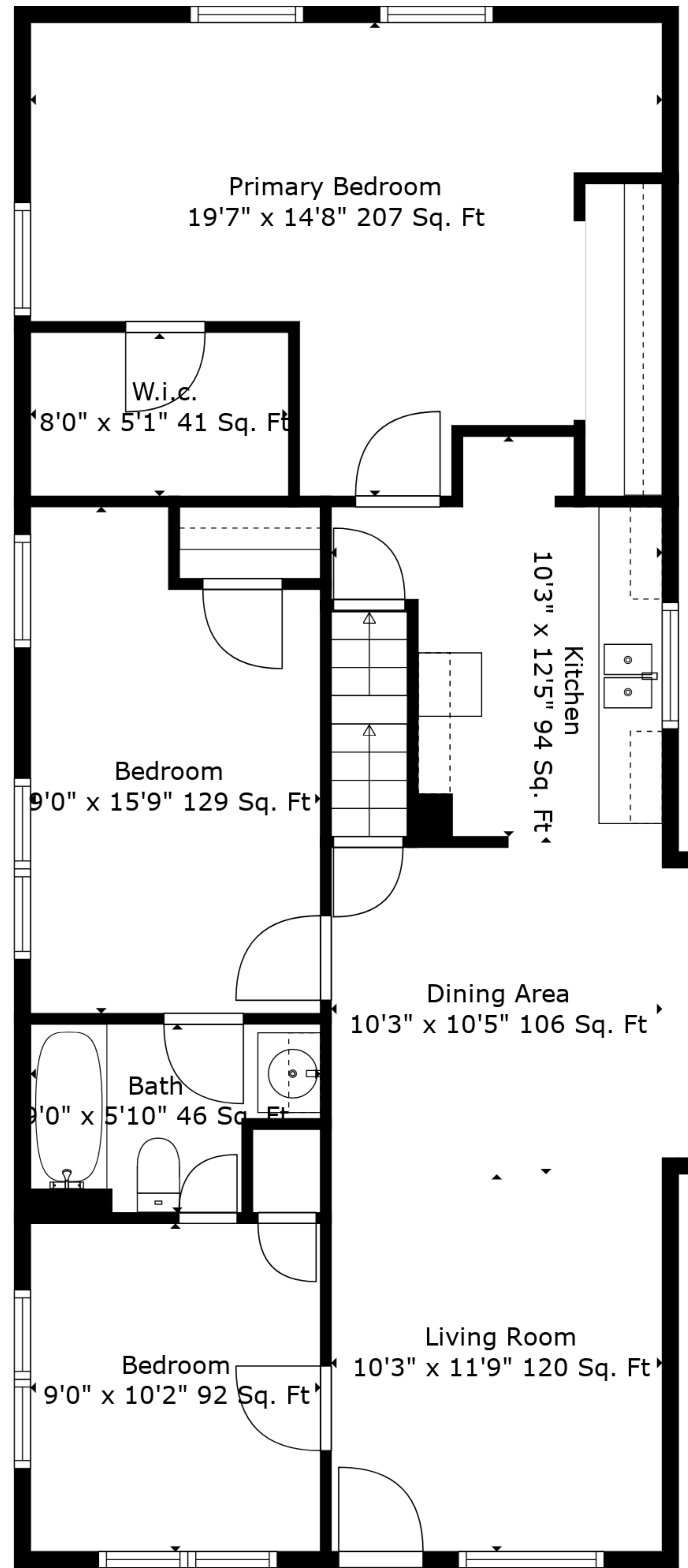
Floor 2
