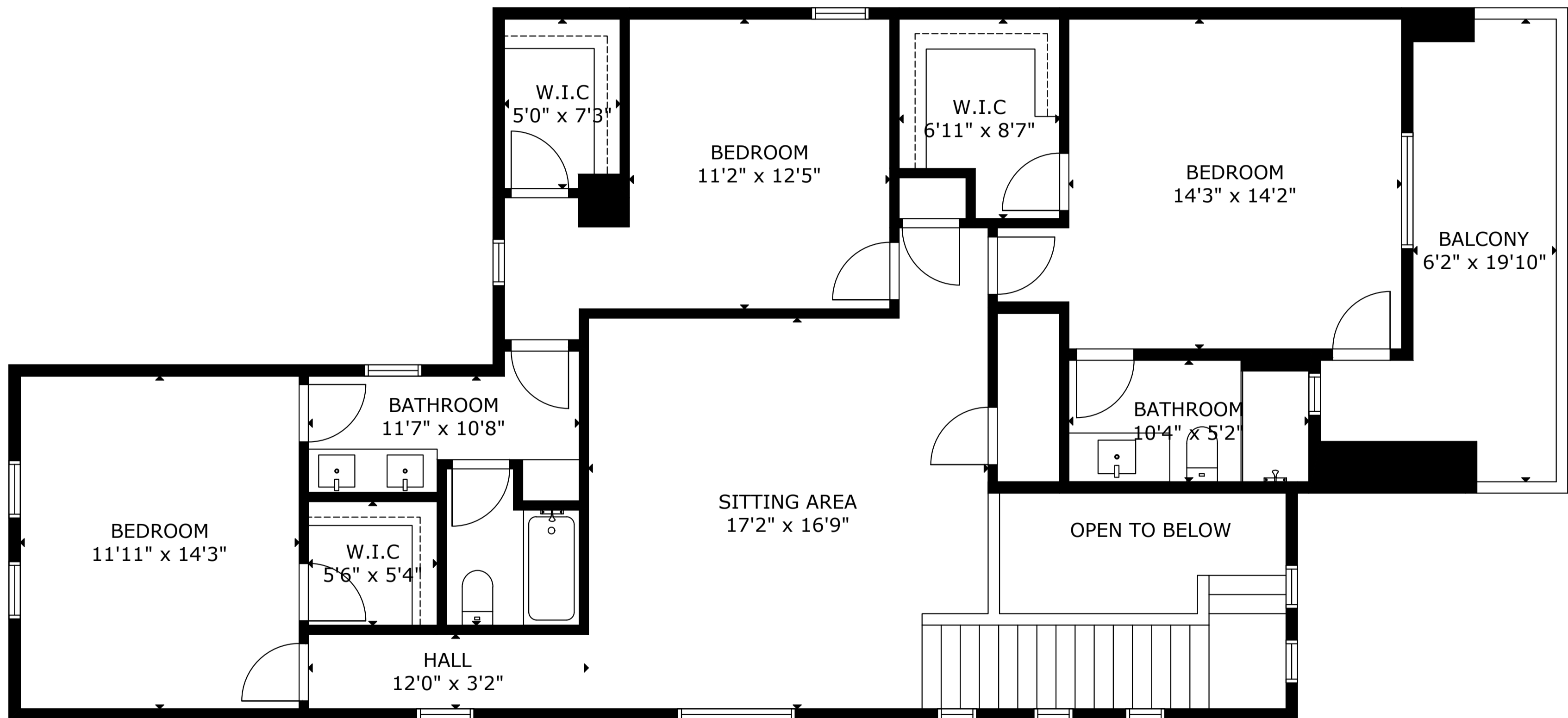
FLOOR 2
