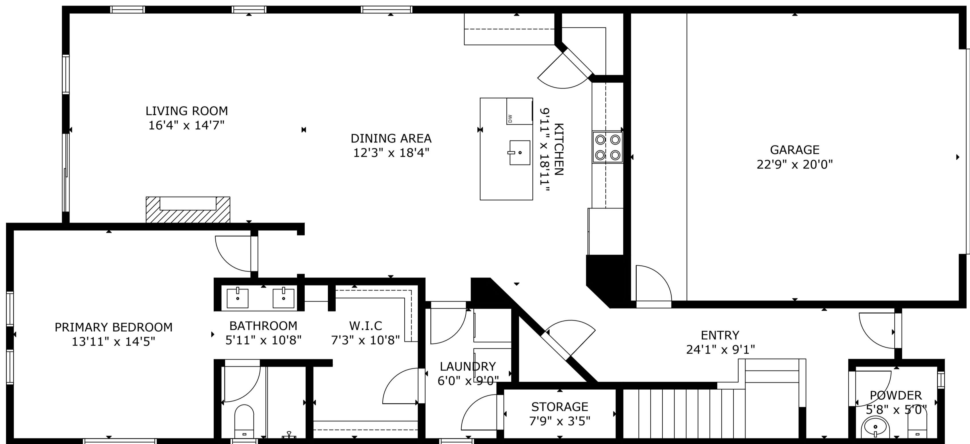
FLOOR 1
