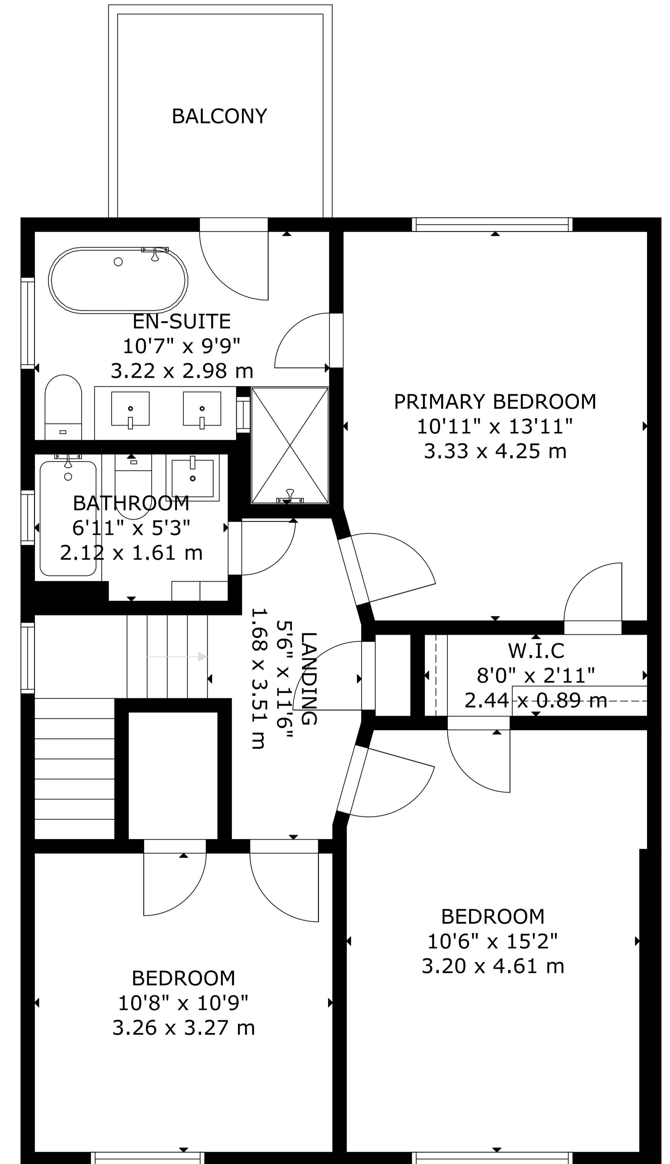
SECOND FLOOR
