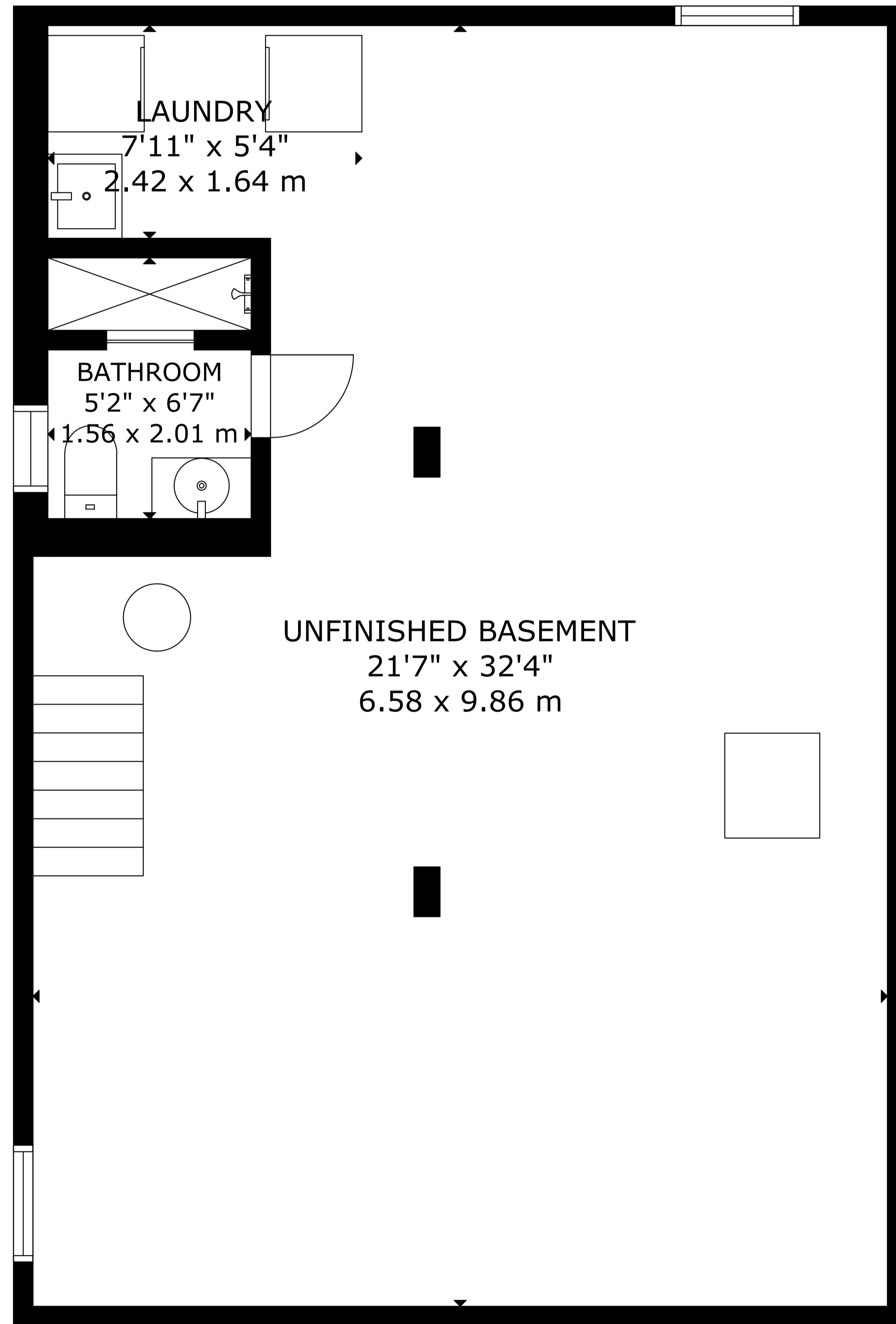
LOWER FLOOR
