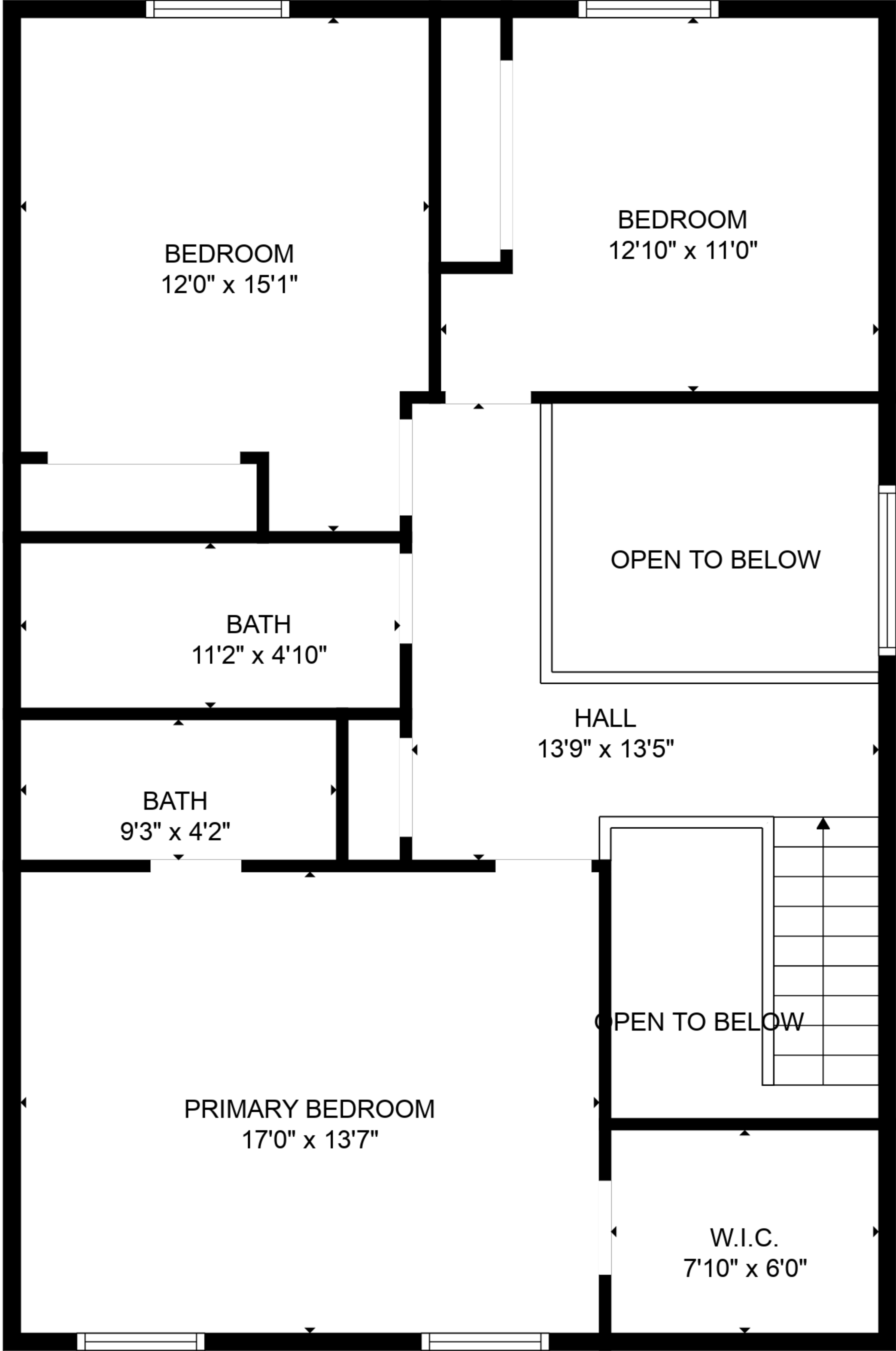
FLOOR 2
