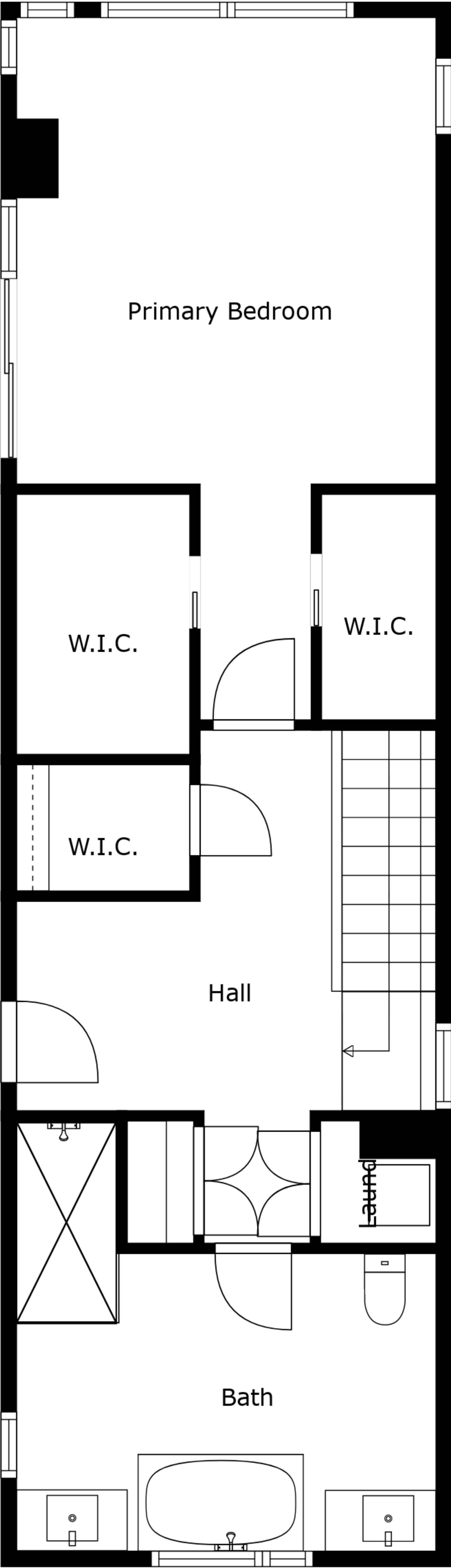
Floor 3
