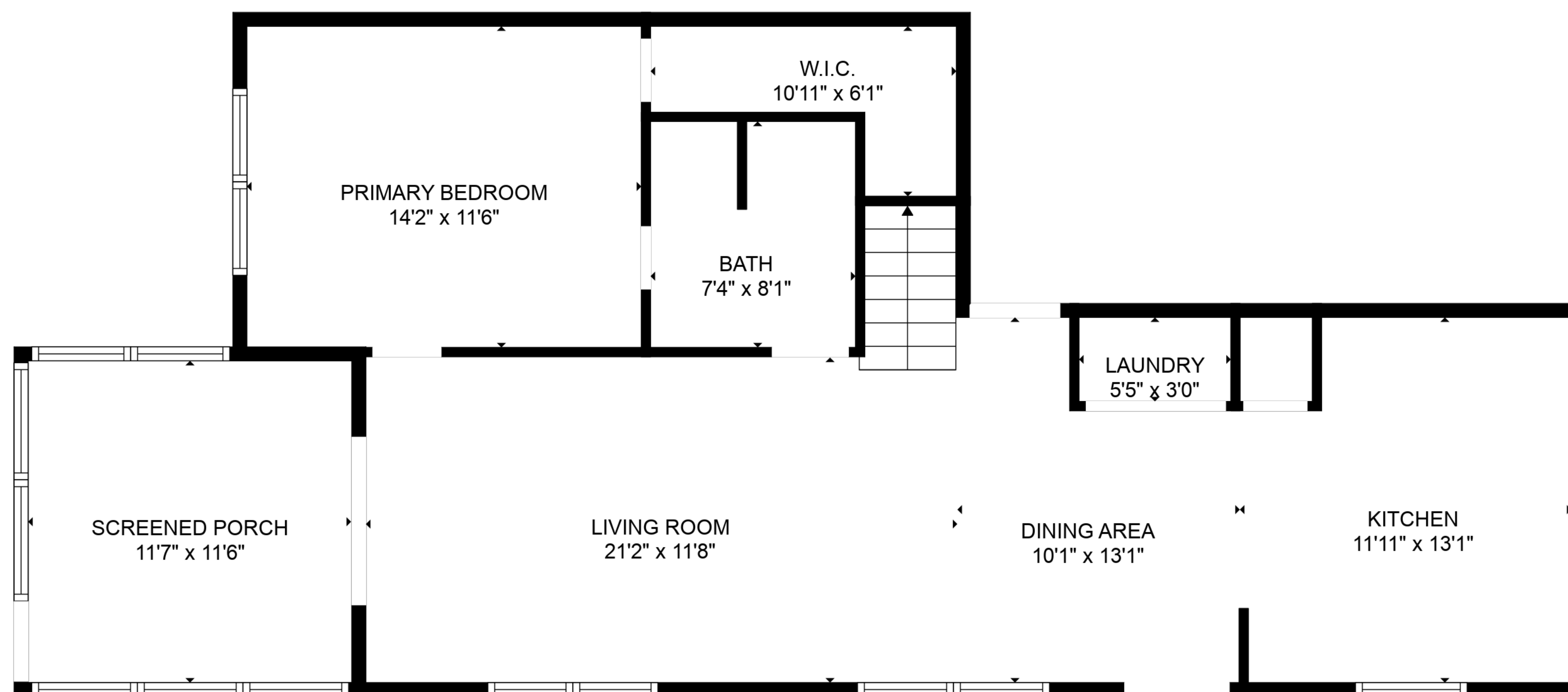
FLOOR 2
