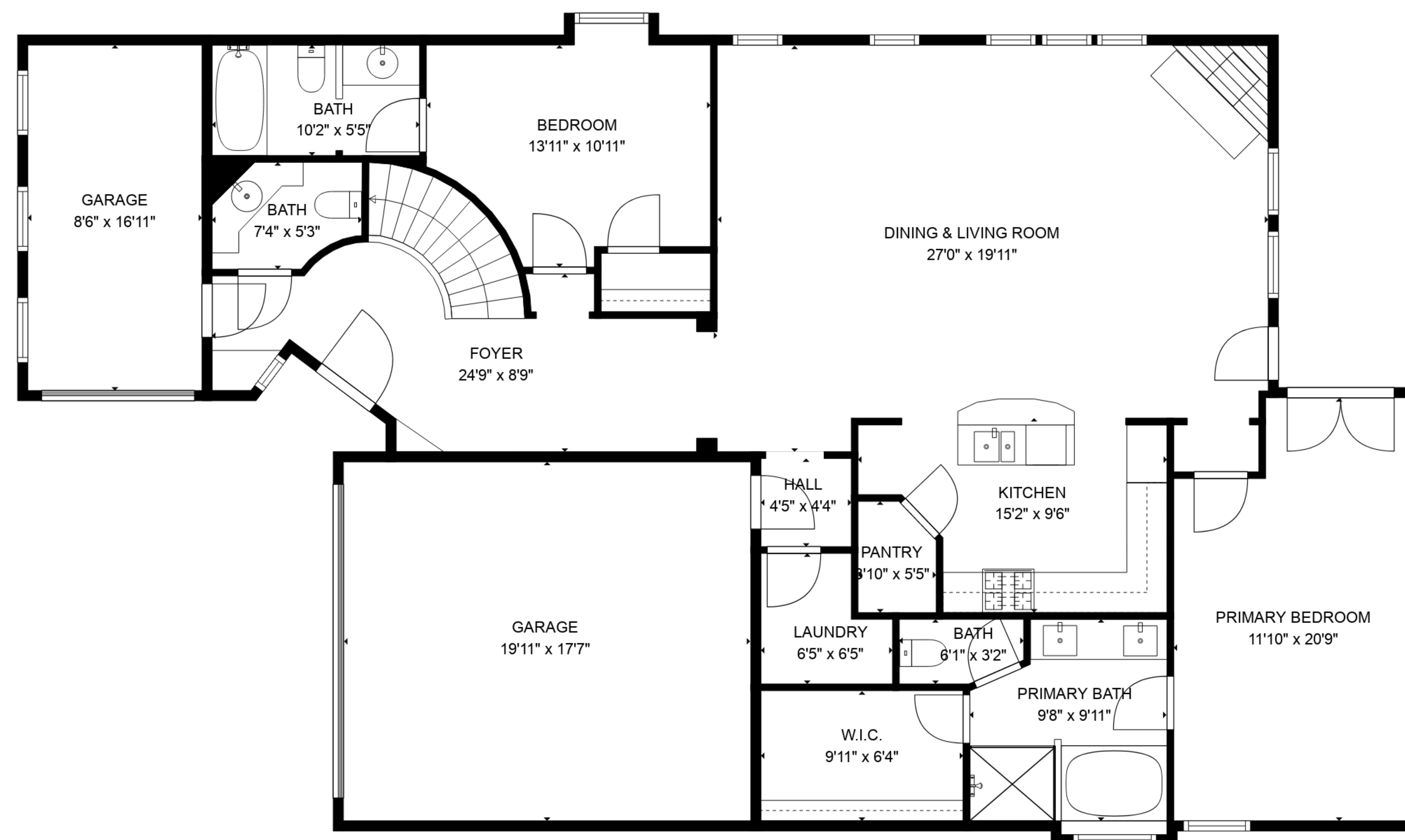
FLOOR 1
