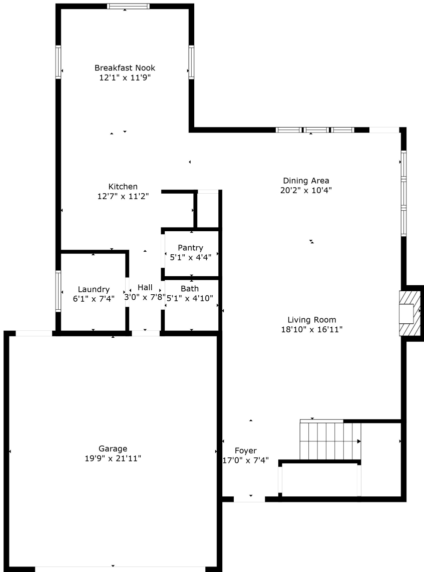
Floor 1
