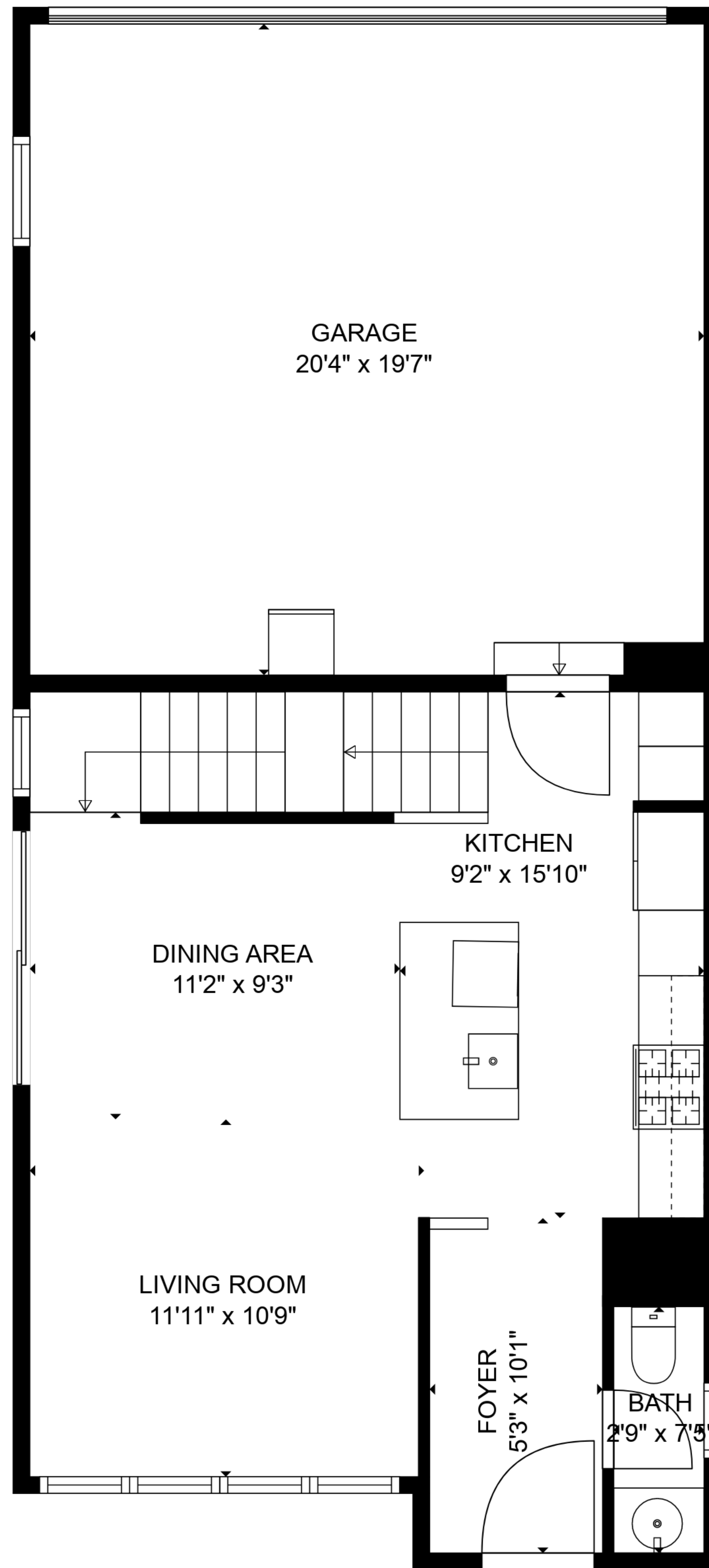
FLOOR 2
