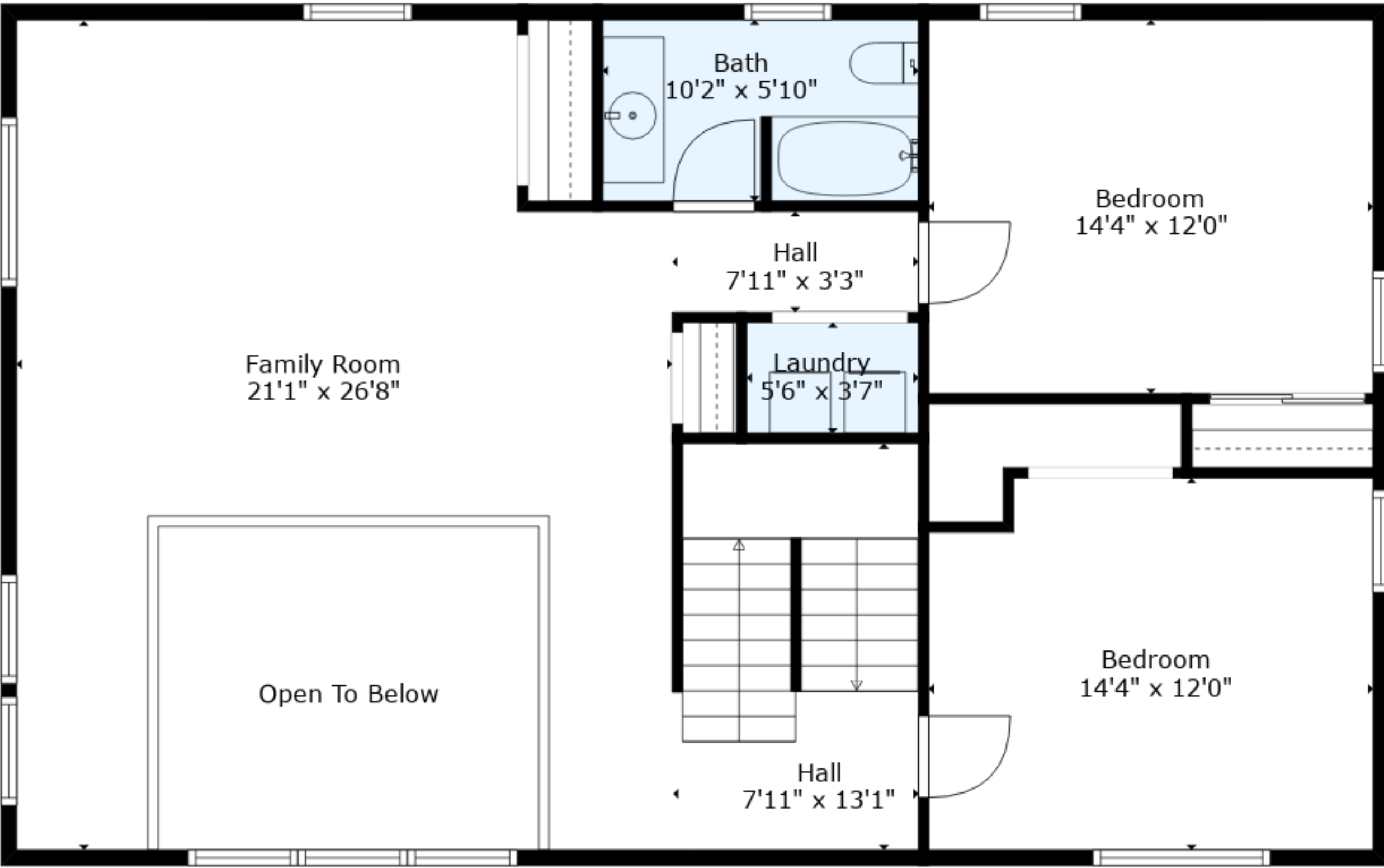
Floor 2
