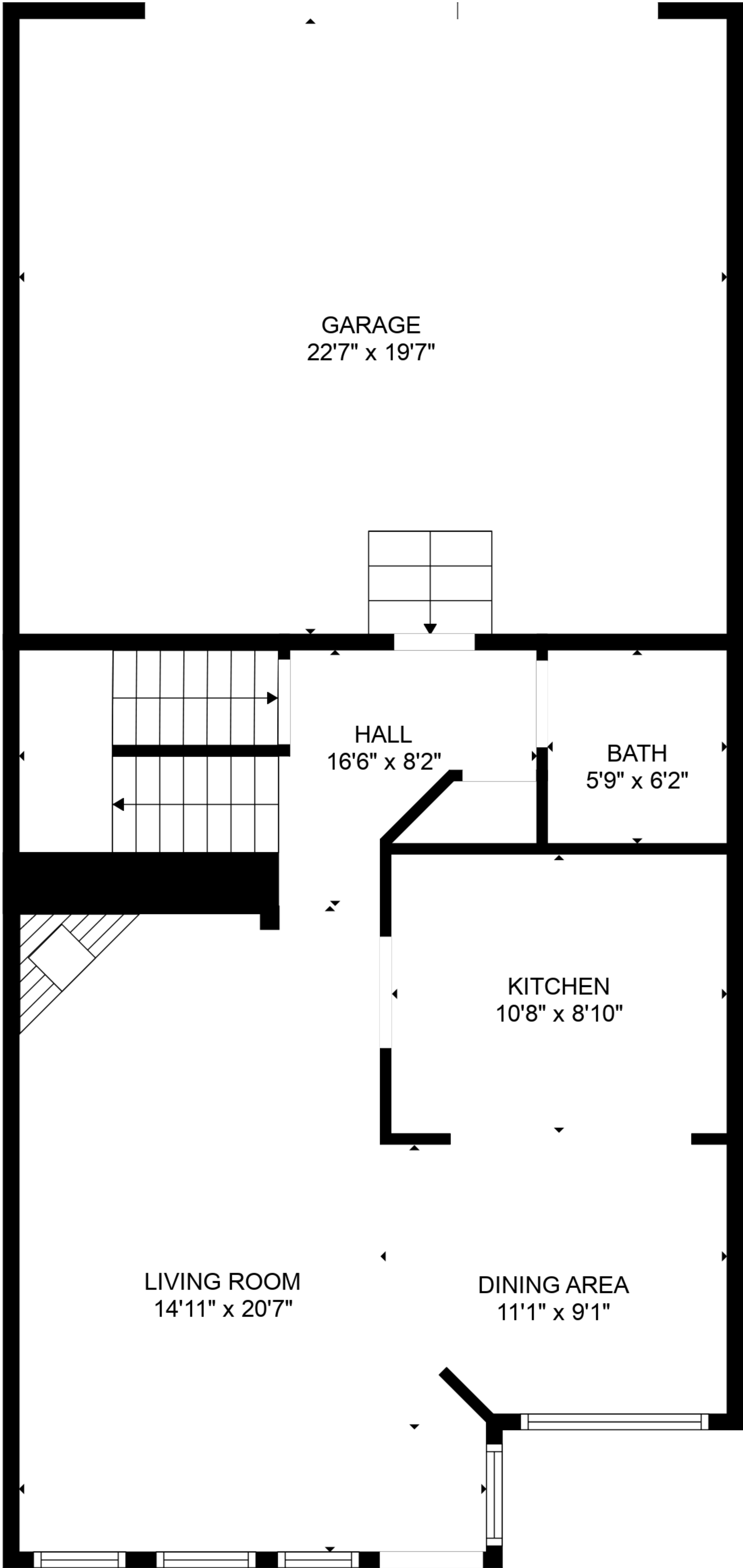
FLOOR 2
