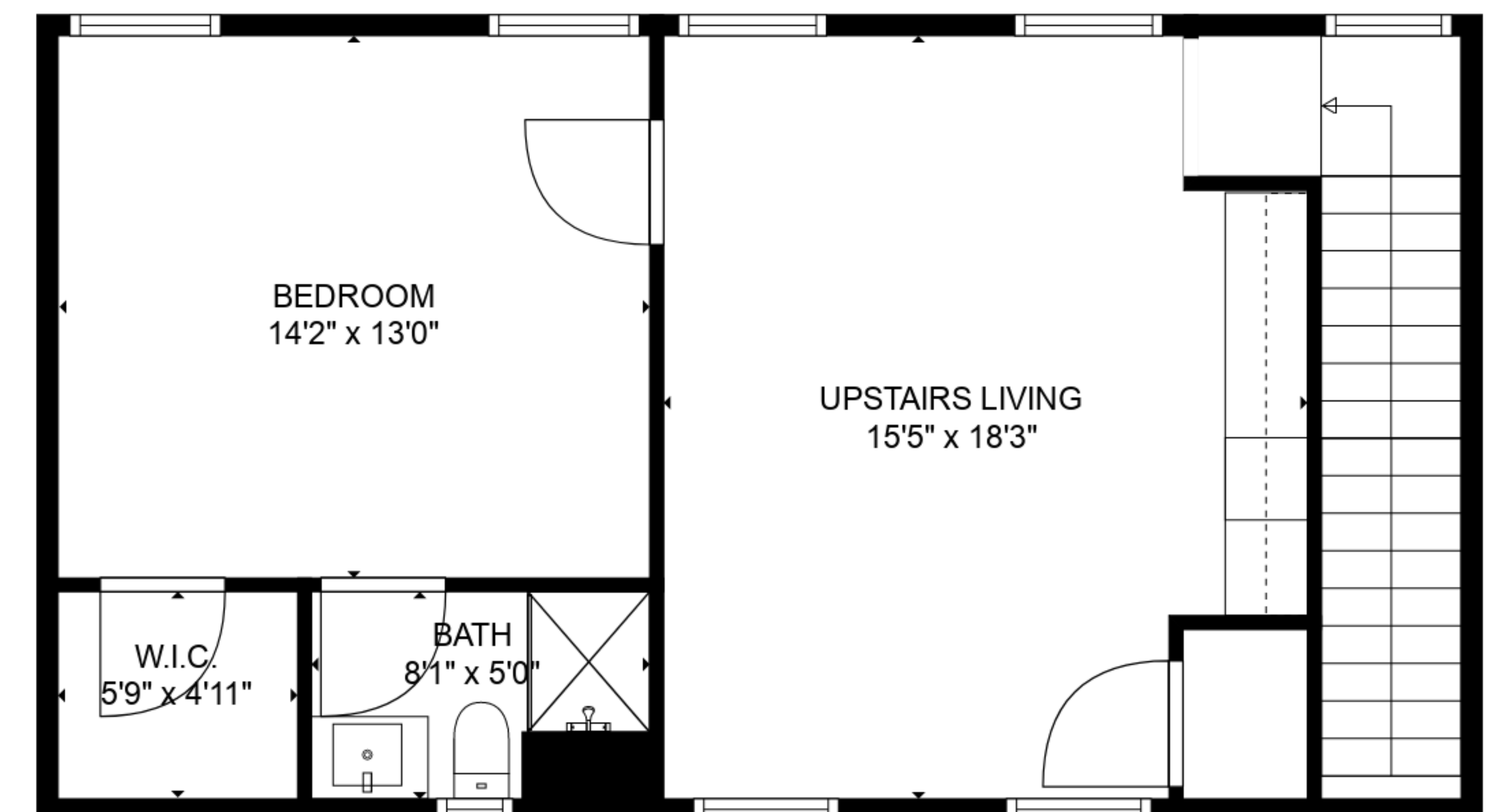
FLOOR 2
