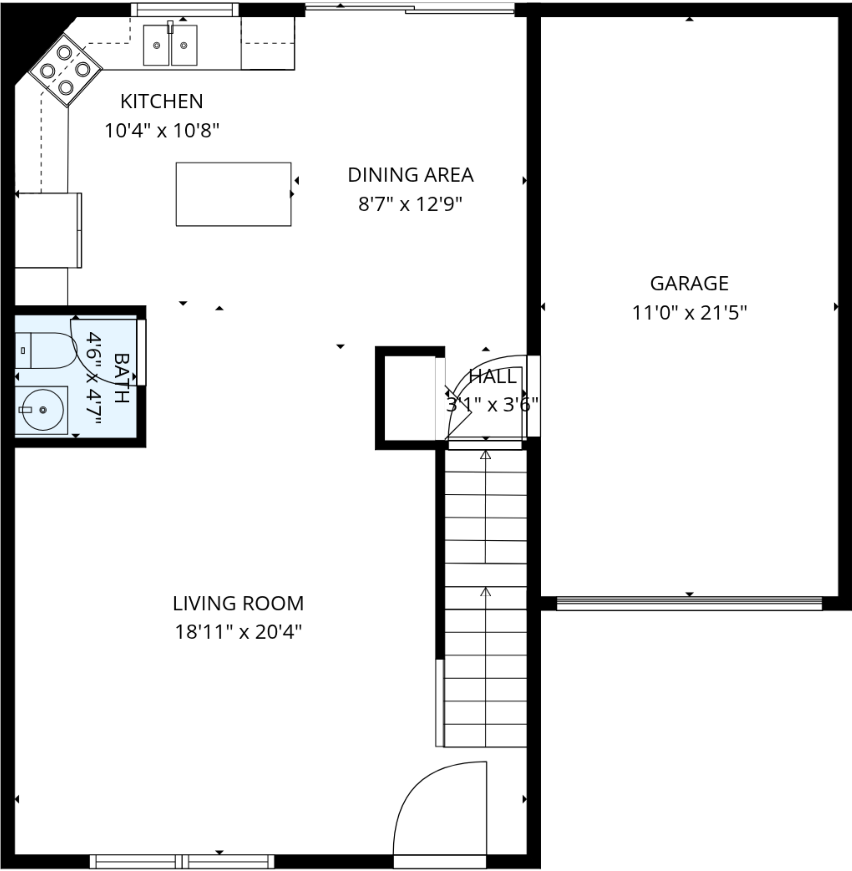
FLOOR 2
