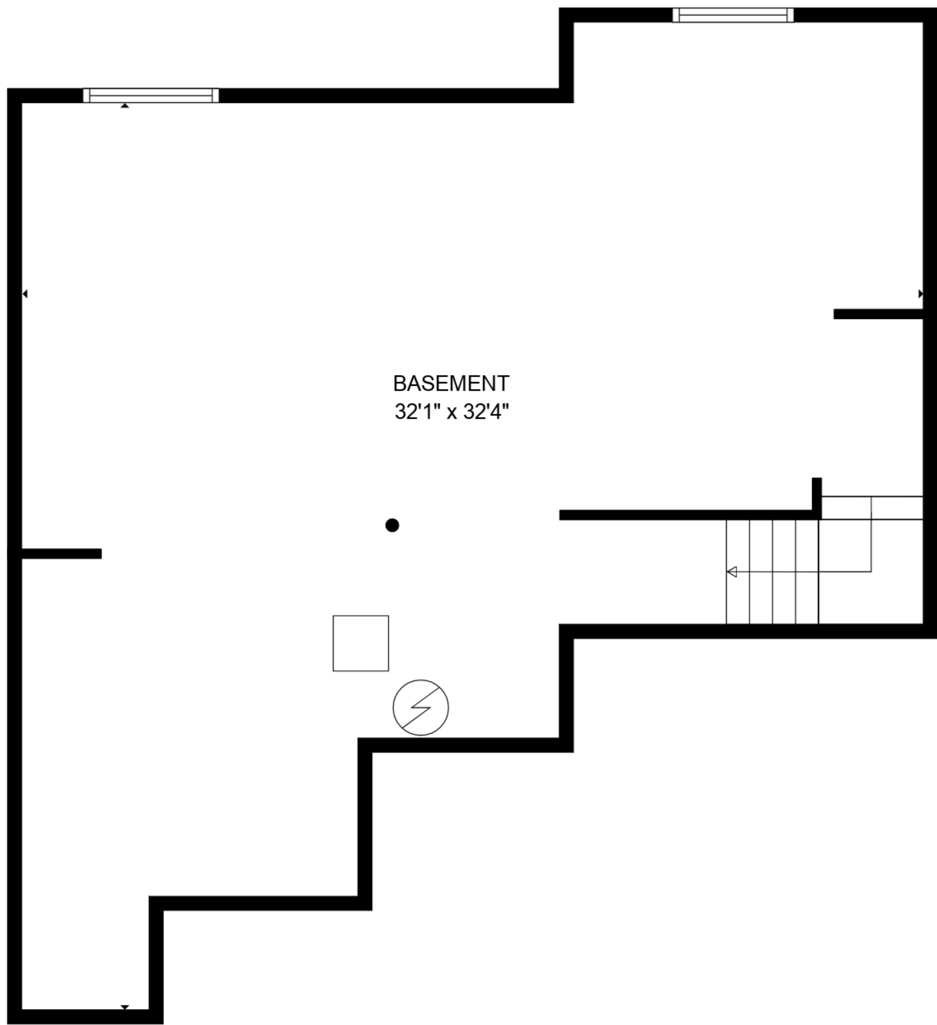
FLOOR 1
