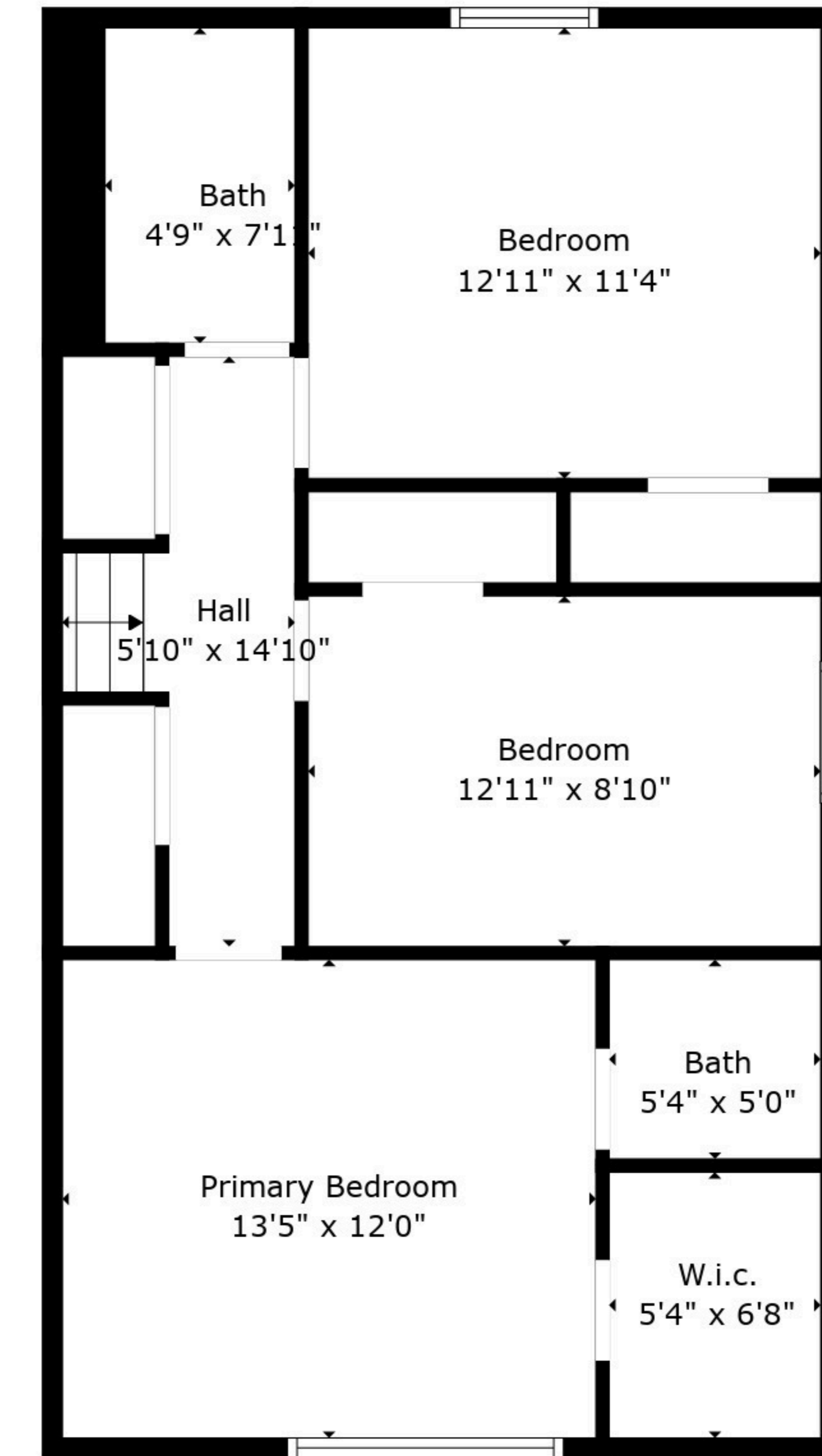
Floor 4
