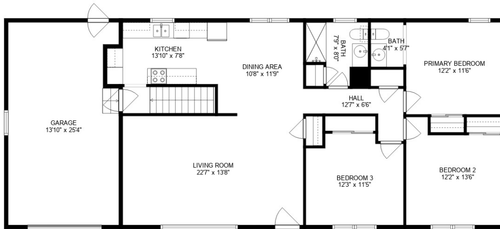
MAIN FLOOR
