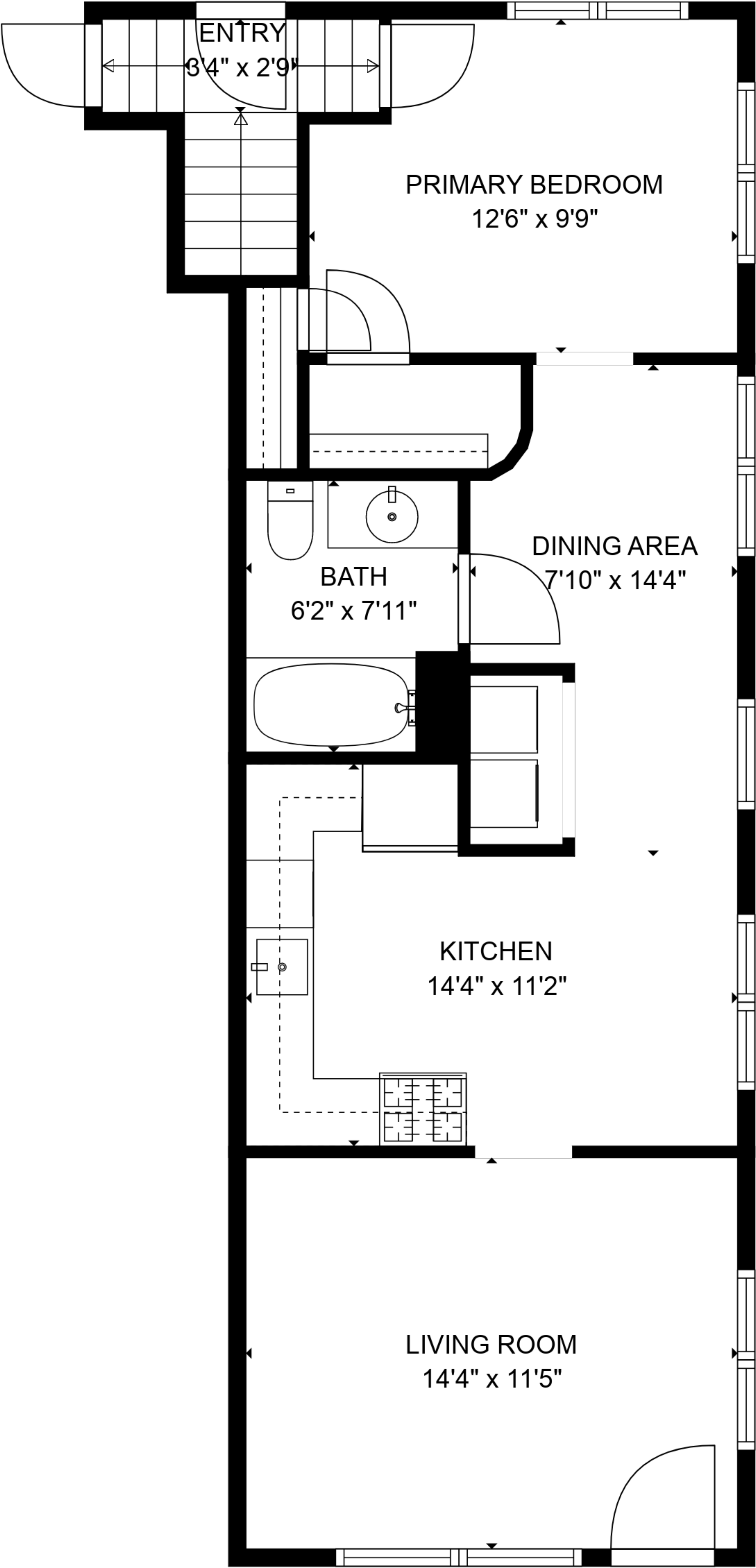
FLOOR 2
