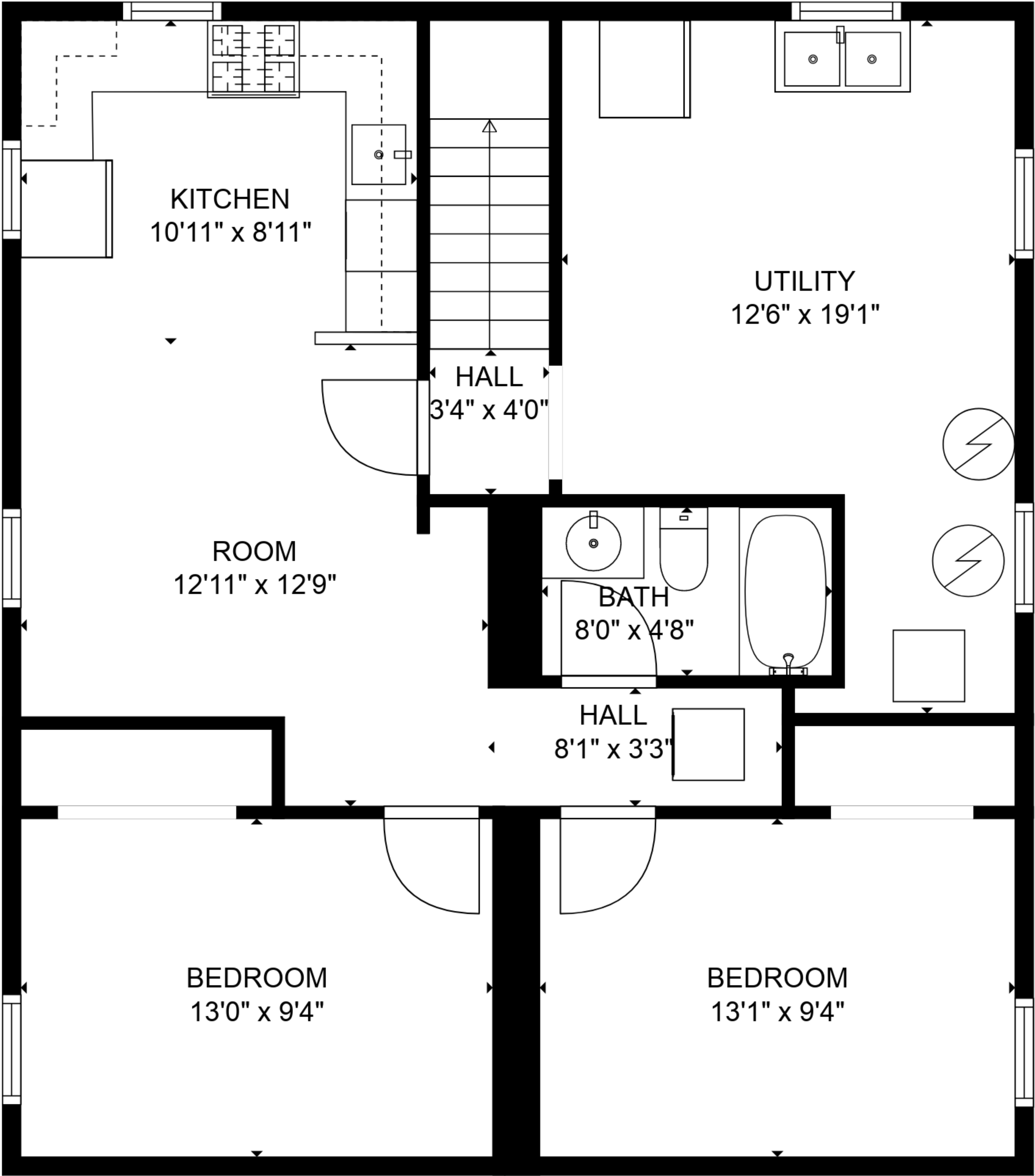
FLOOR 1
