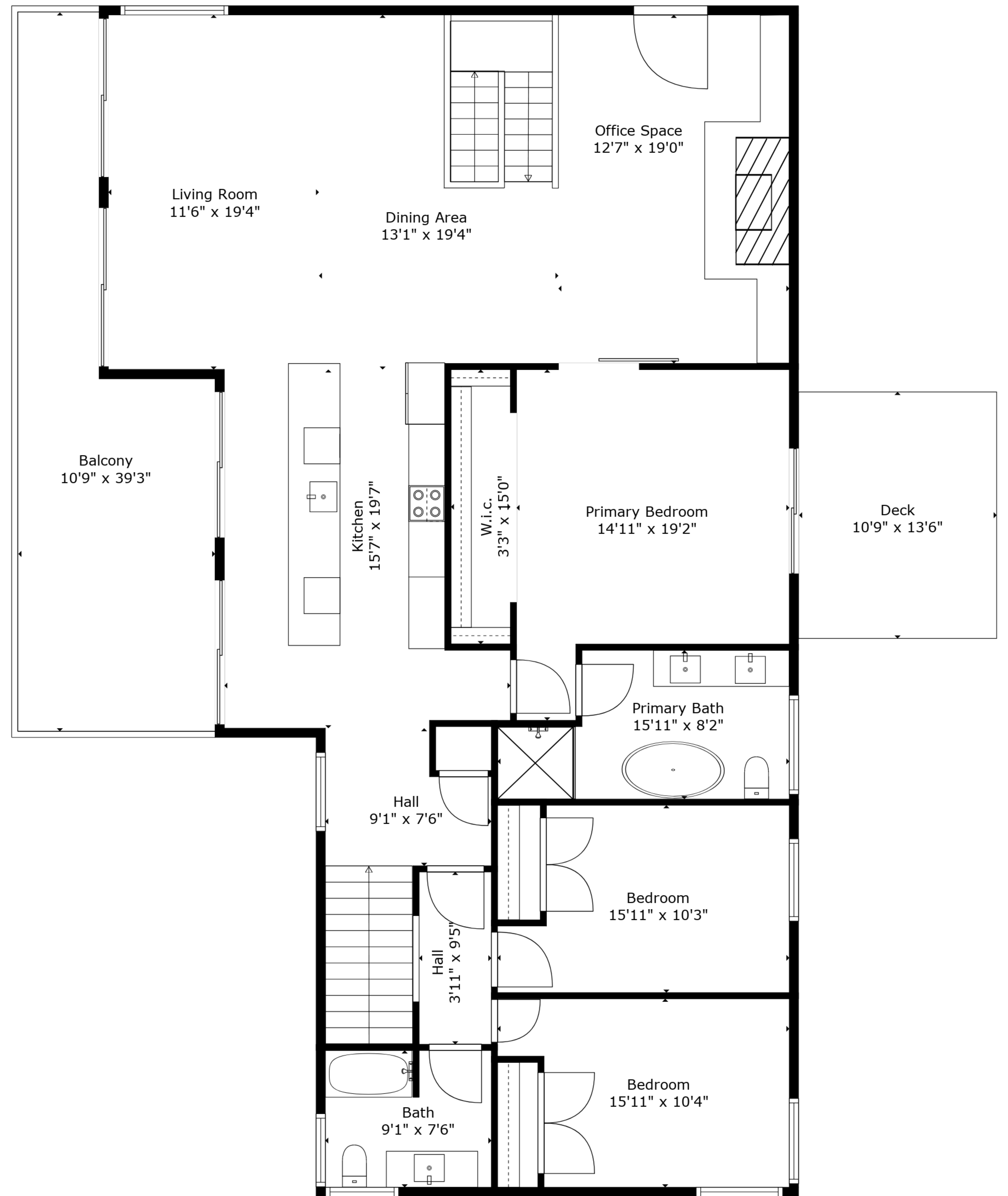
Floor 2
