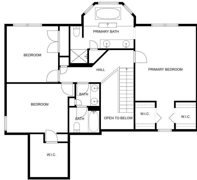
FLOOR 3
