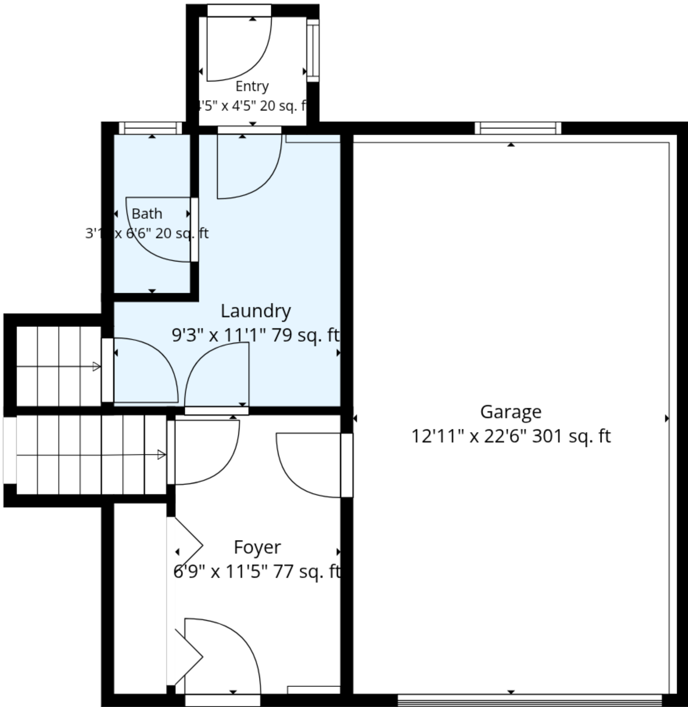
1st Floor
