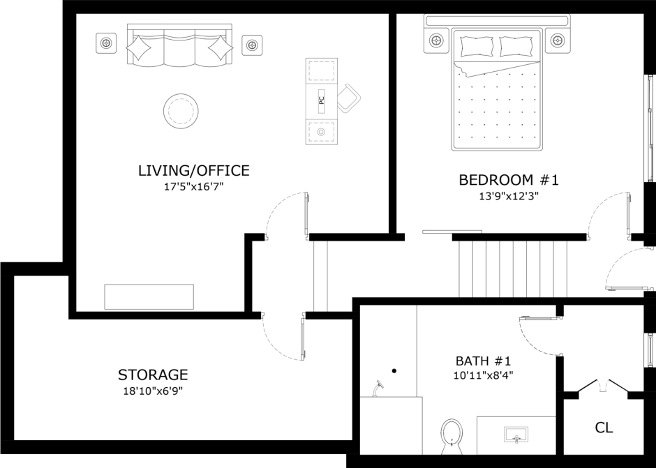
FLOOR-1
