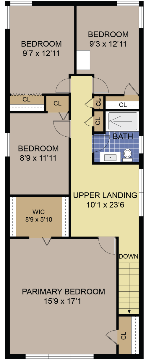
THIRD FLOOR
