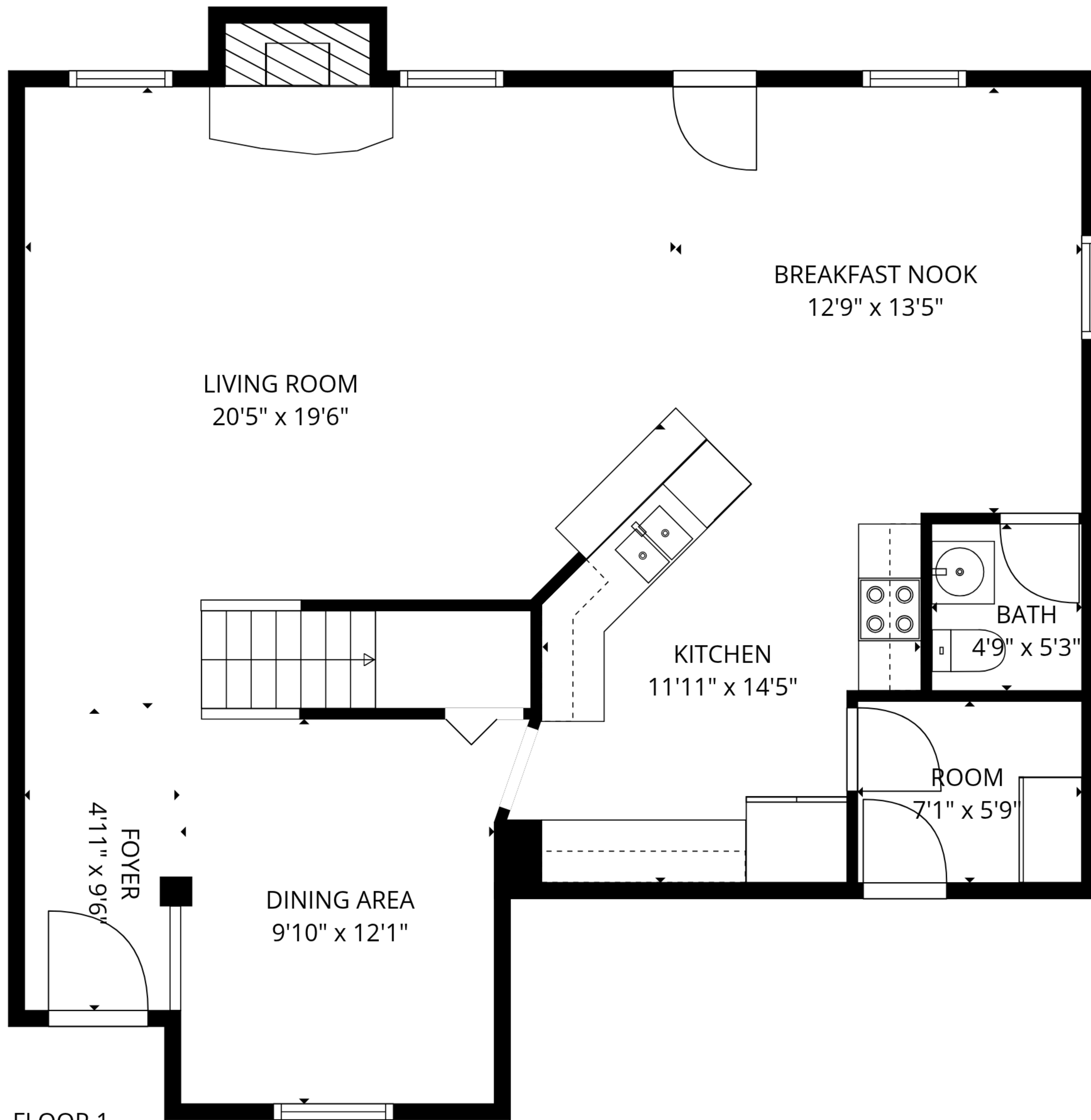
FLOOR 1
