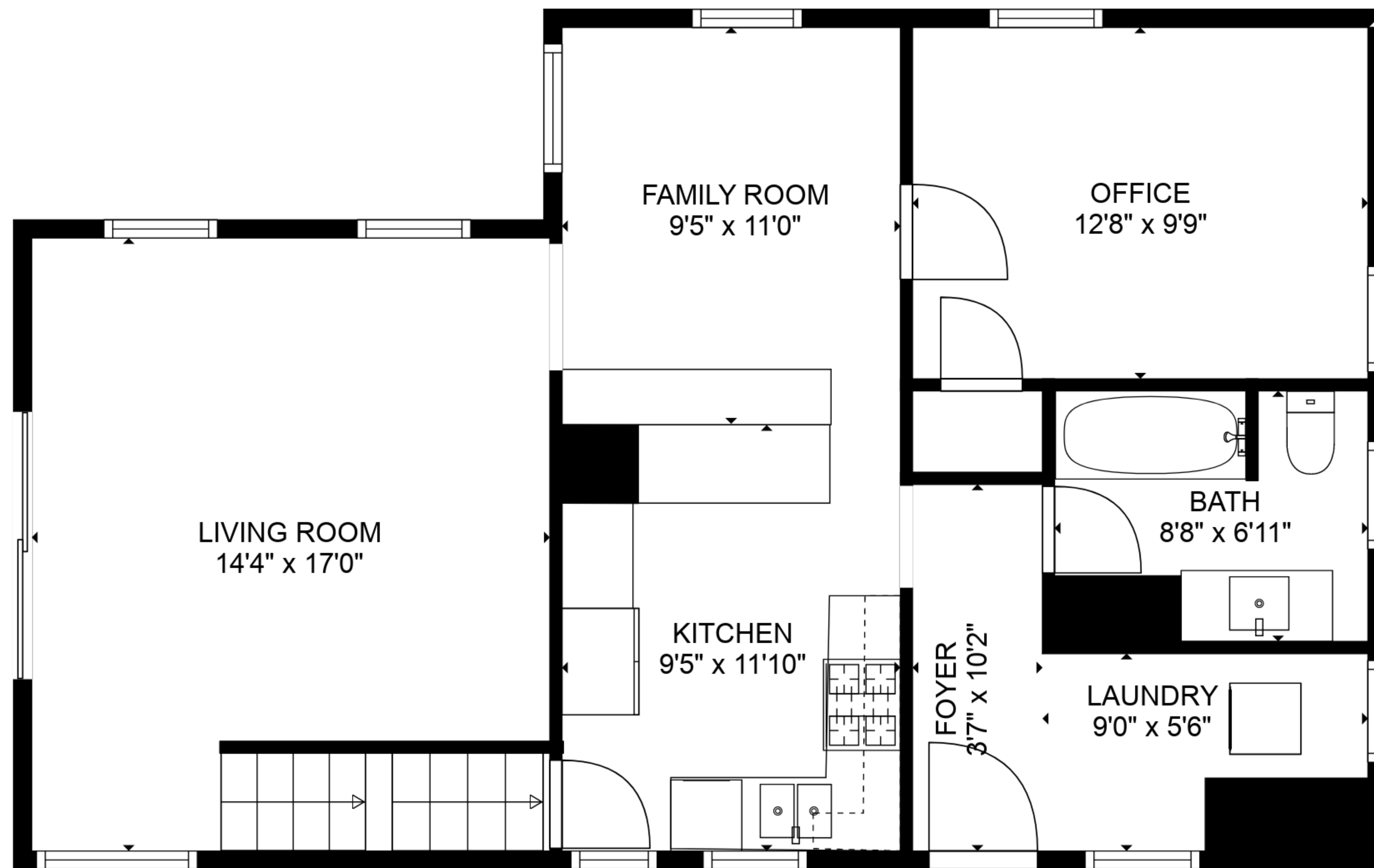
FLOOR 2
