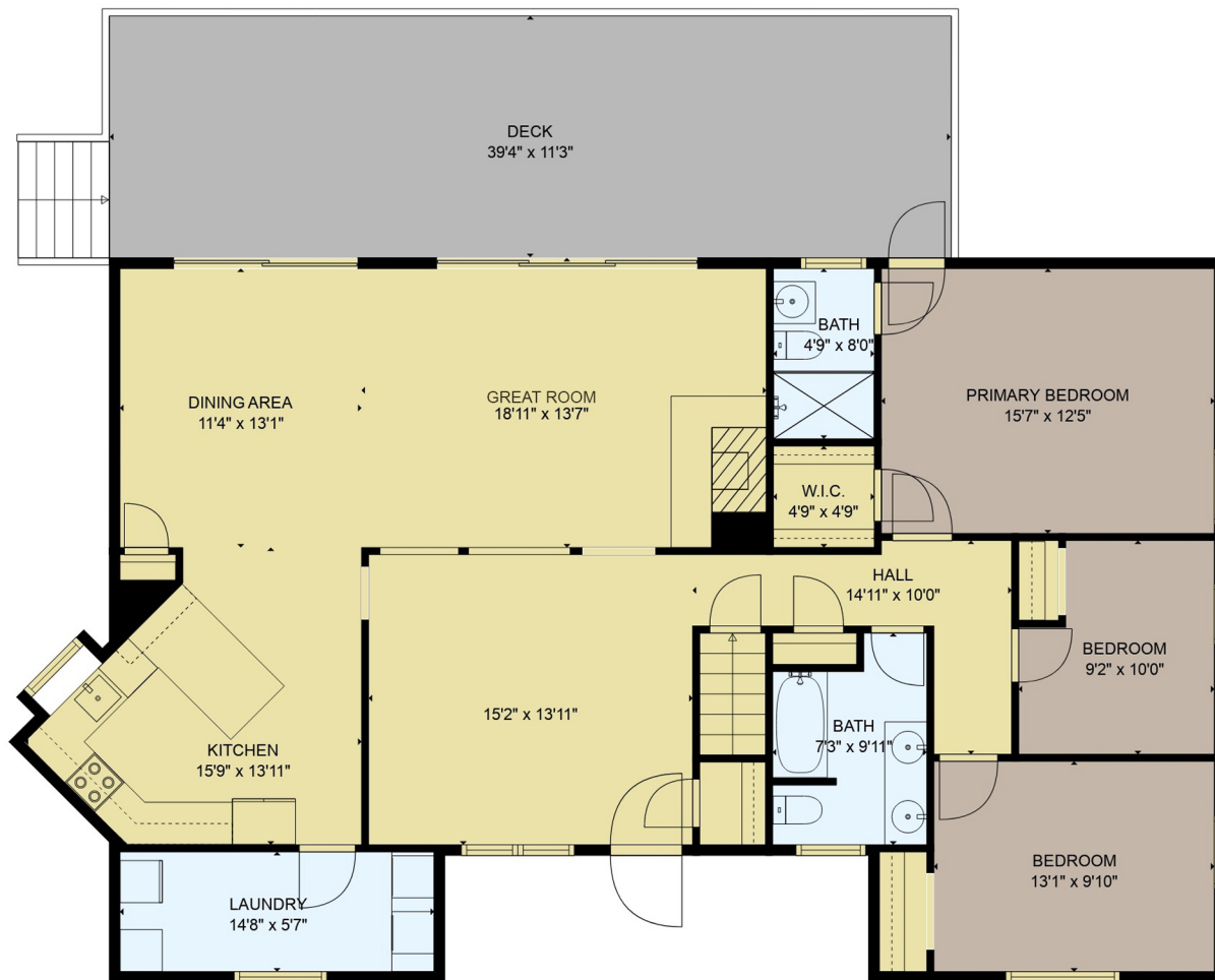
MAIN LEVEL
