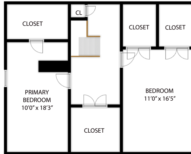
TOP LEVEL 768 SQ.FT
