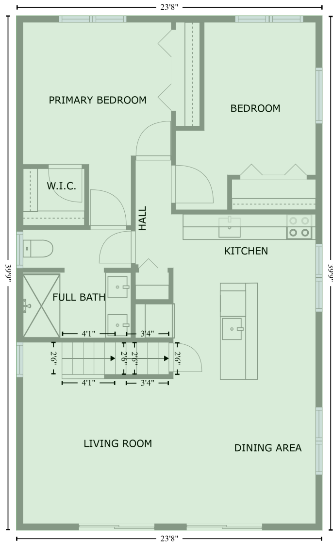
FLOOR 2 [AREA: 940]
