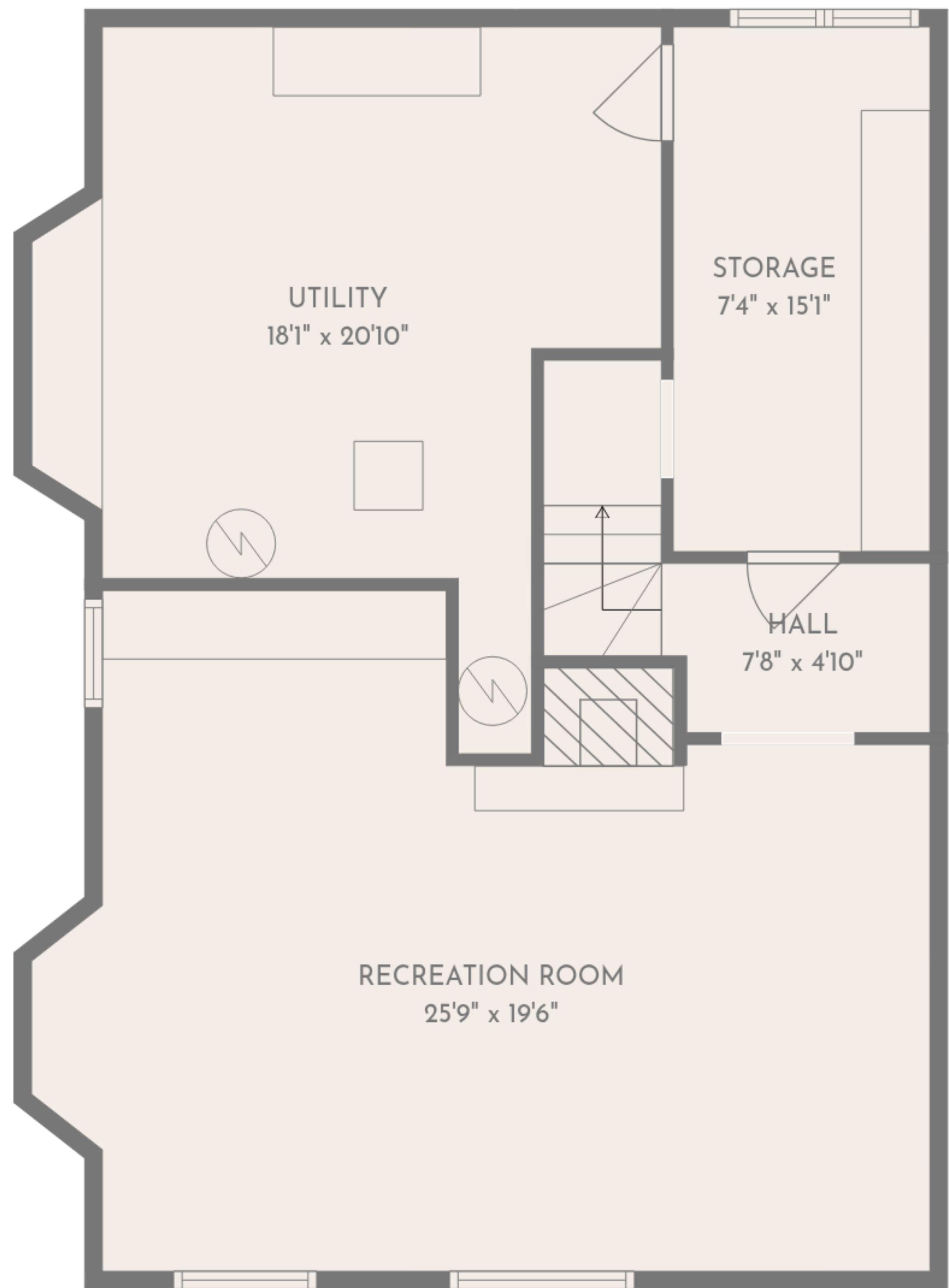
Basement 1
