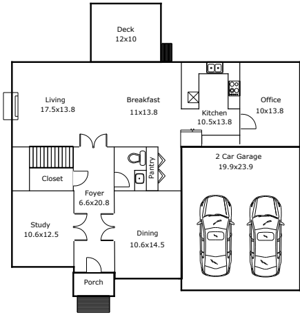
1st Floor
