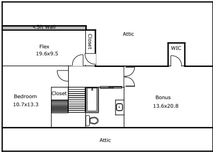
3rd Floor
