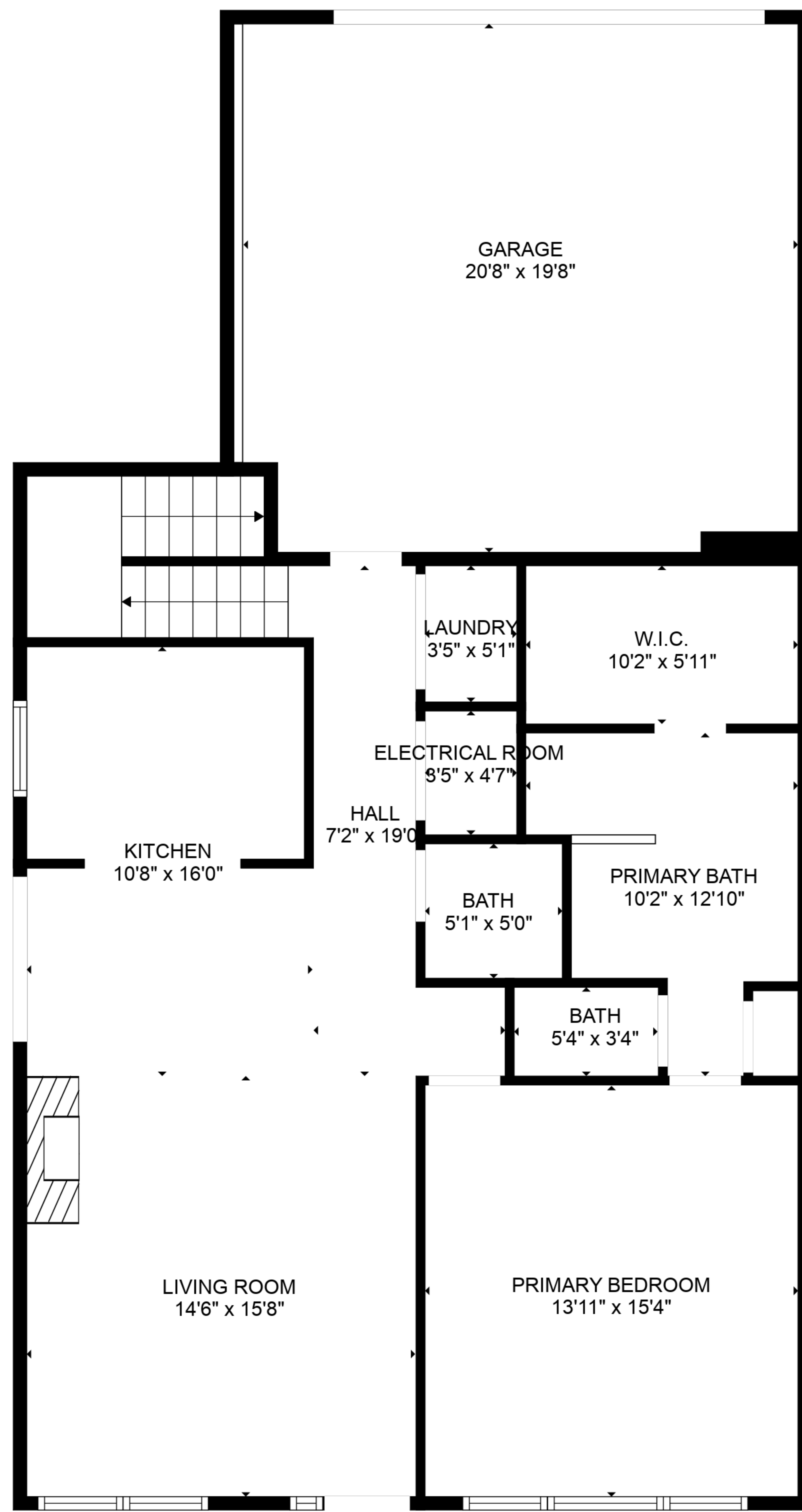
FLOOR 1
