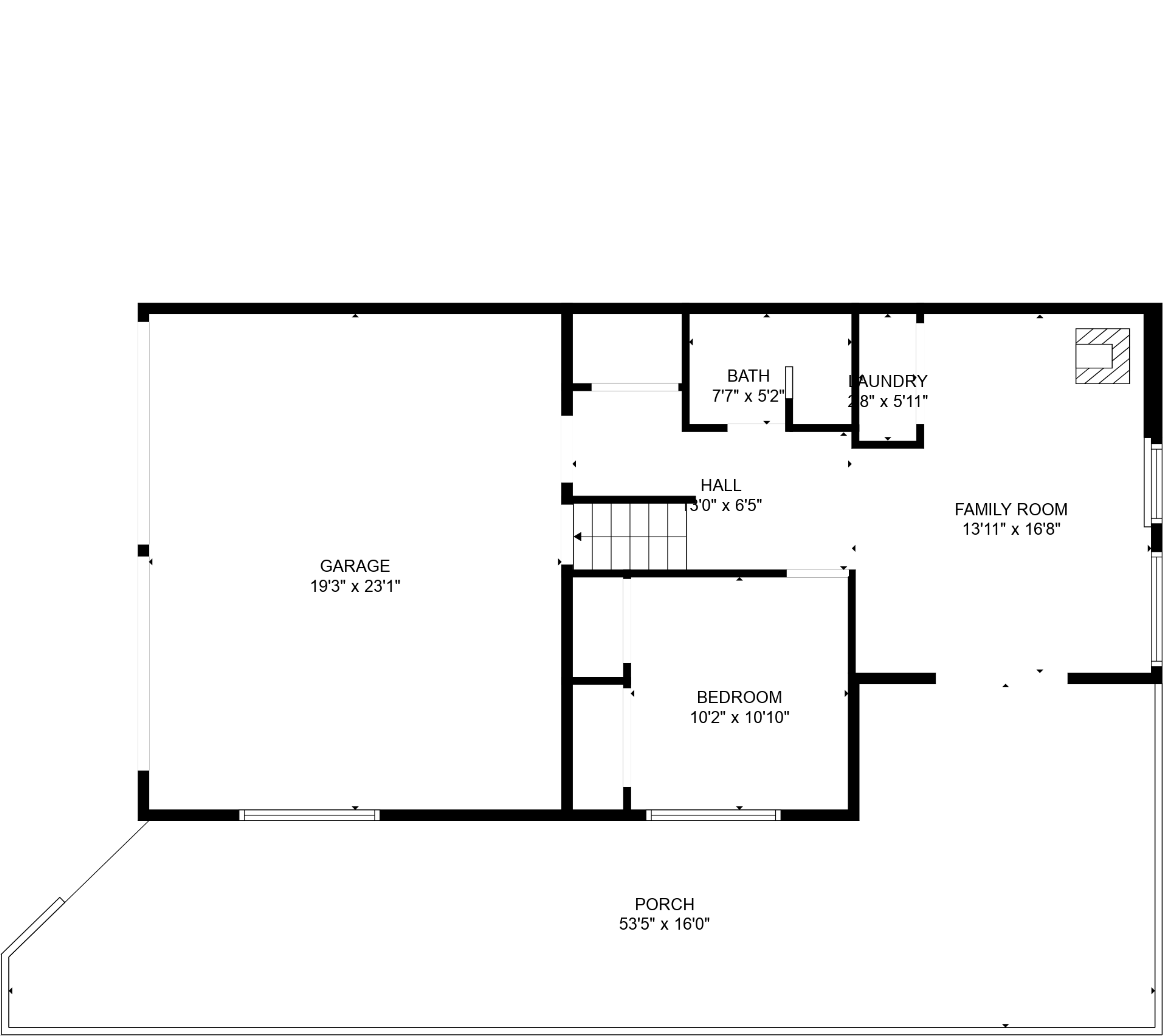
FLOOR 1
