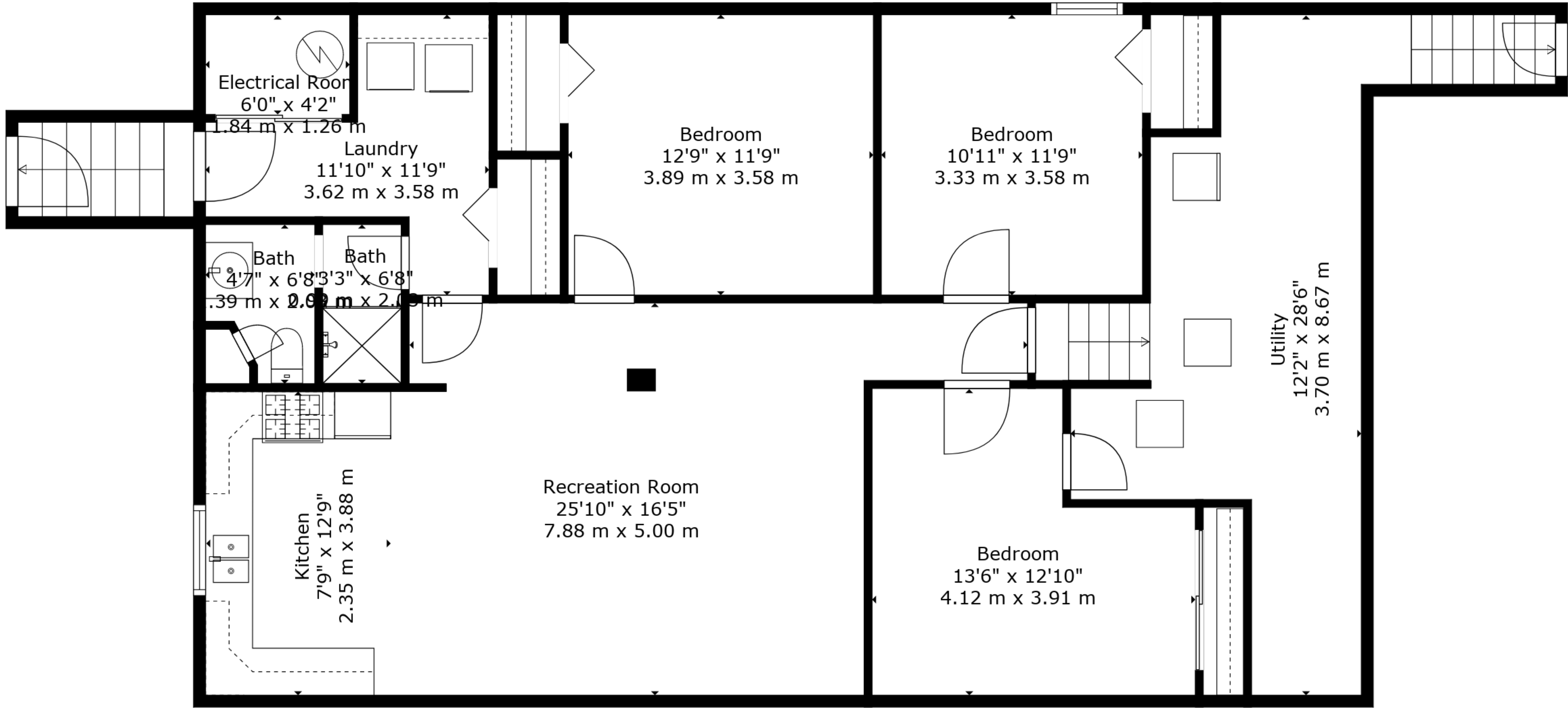
Floor 1
