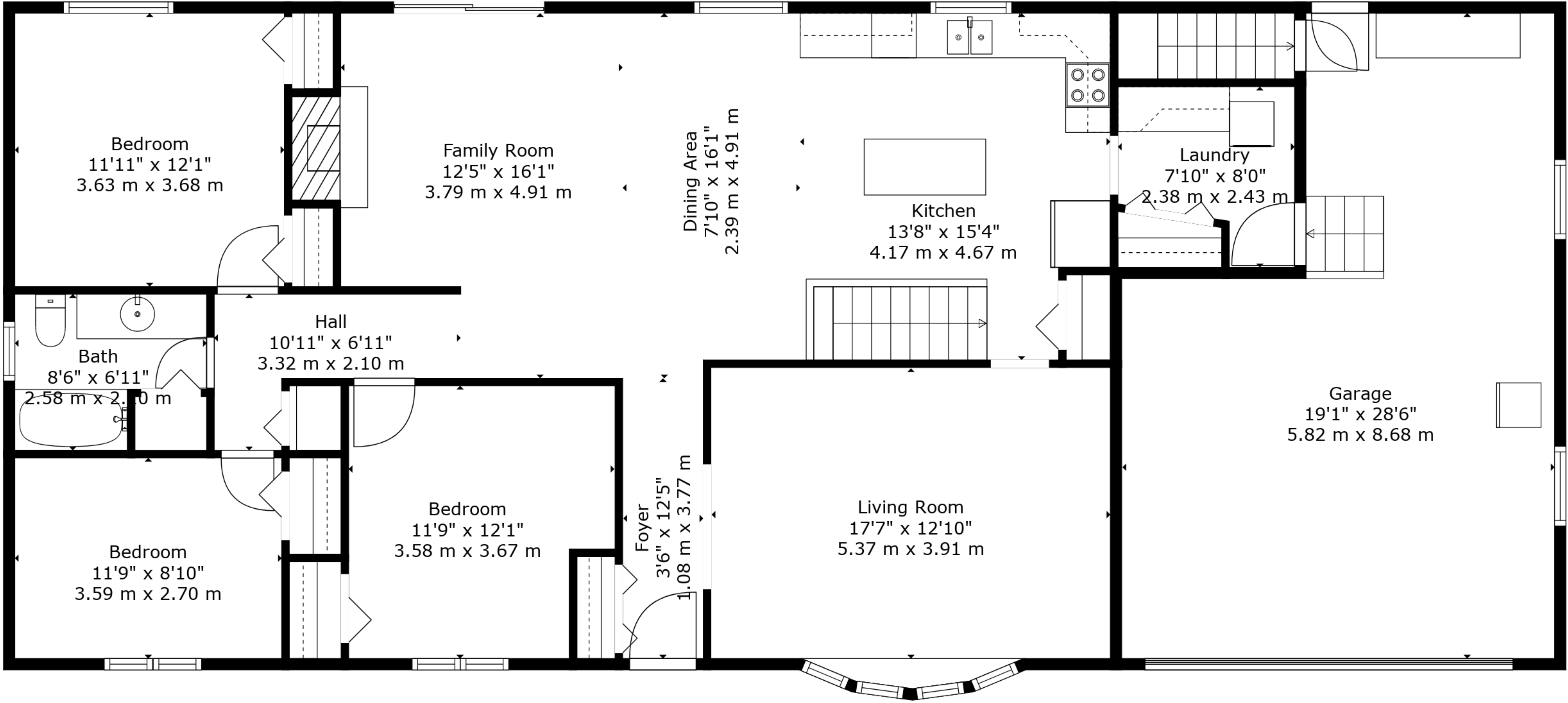
Floor 2
