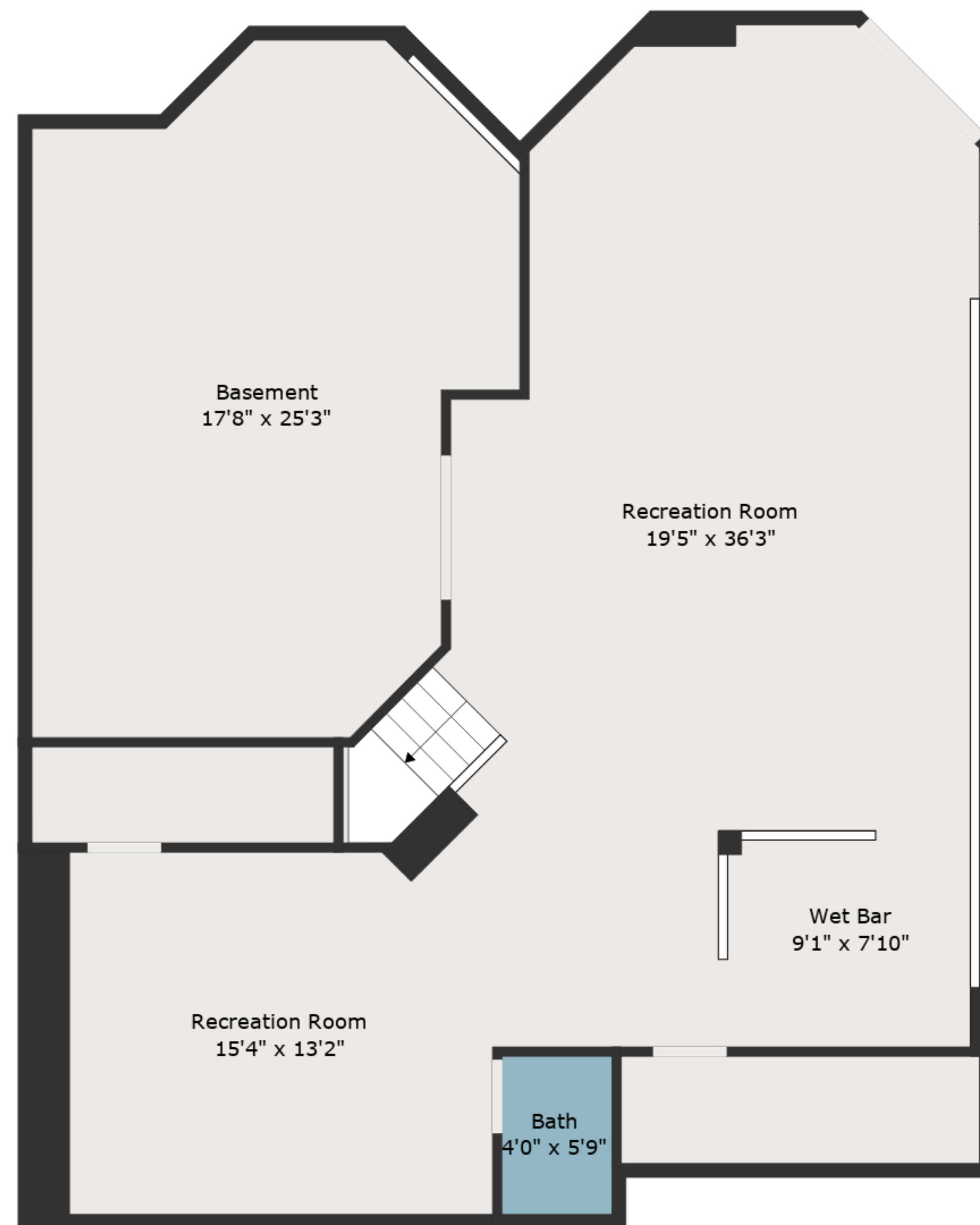
Floor 1
