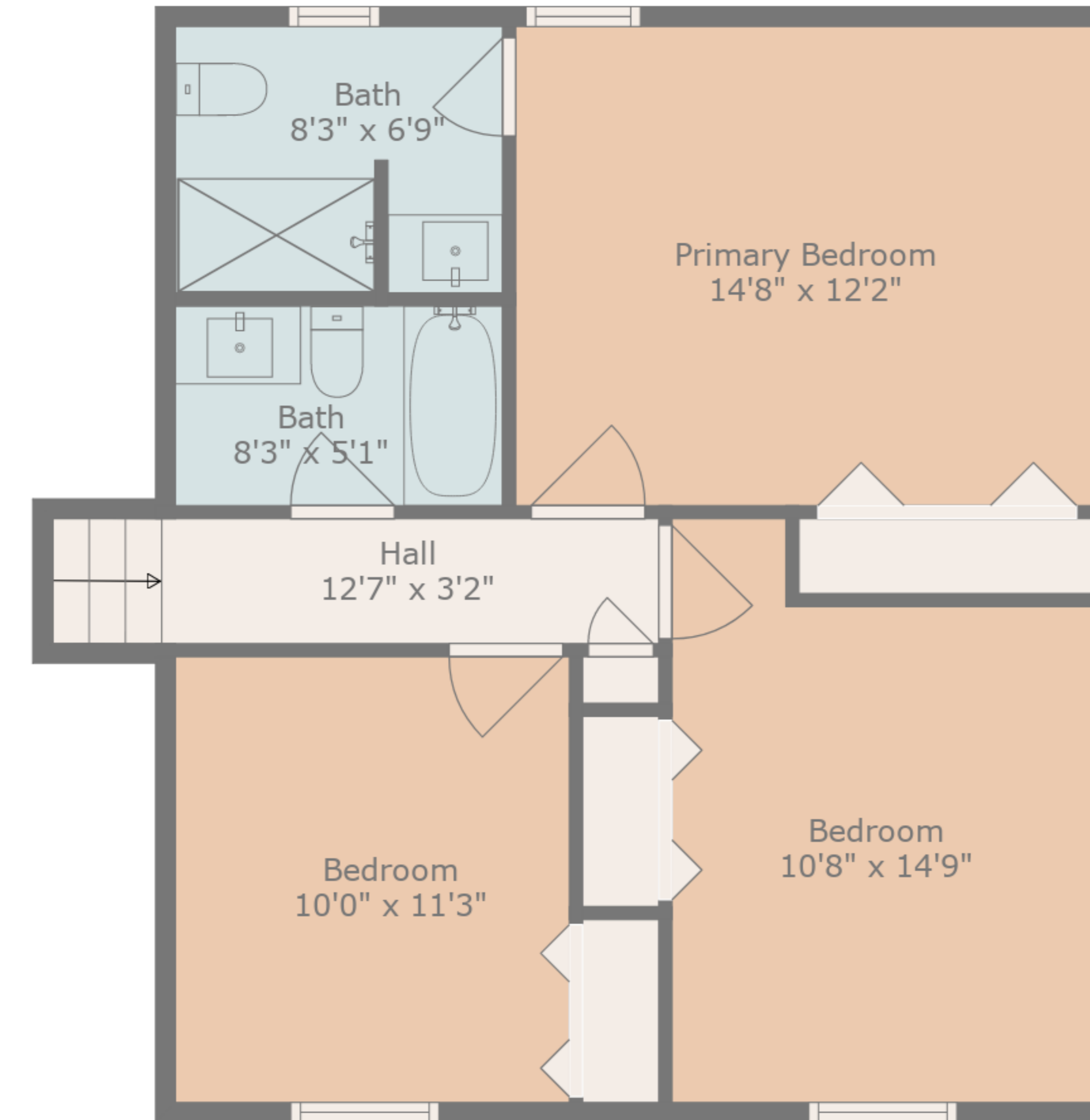
Floor 4
