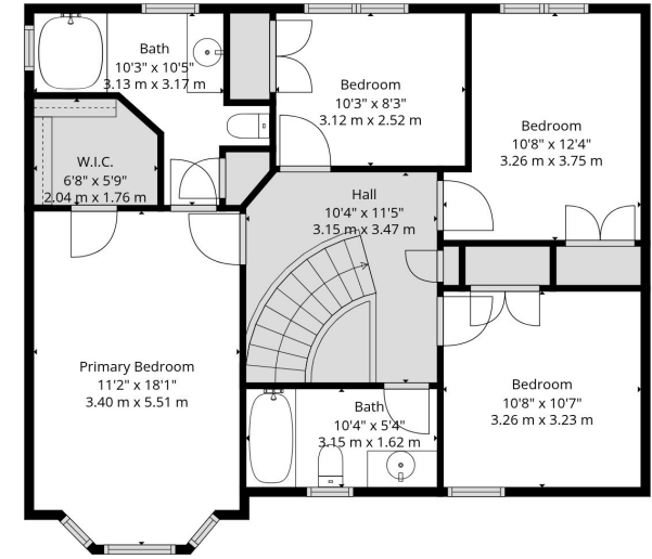
2nd Floor
