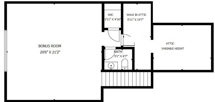
2ND FLOOR
