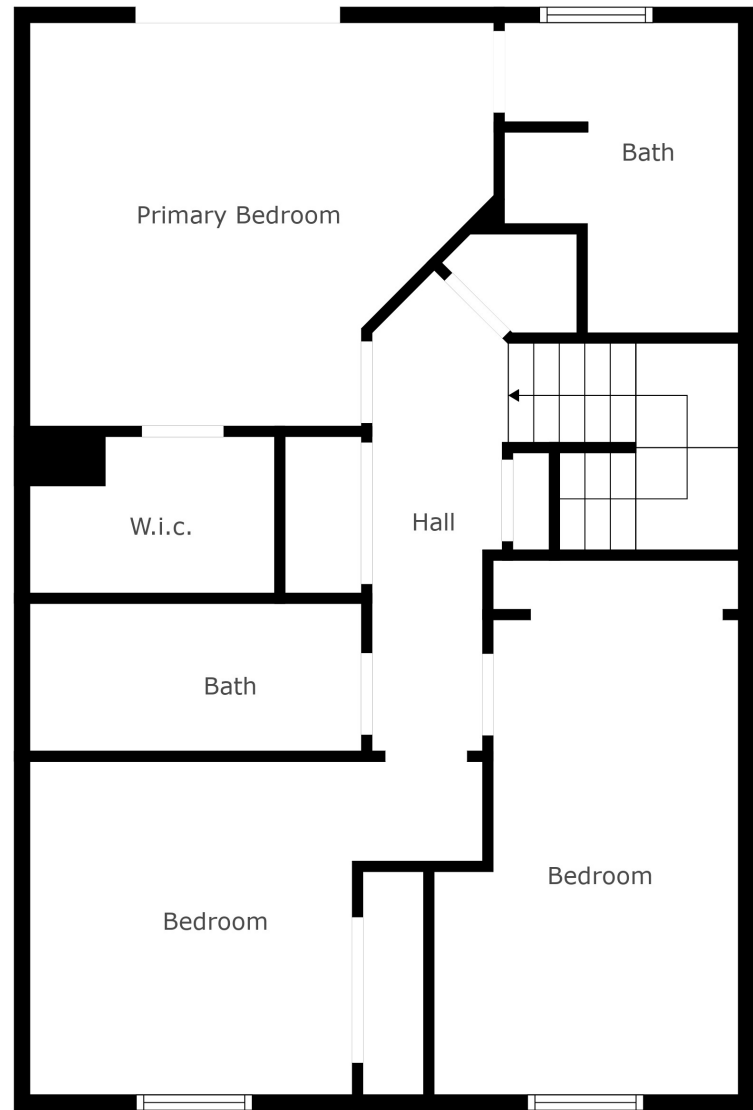
Floor 2
