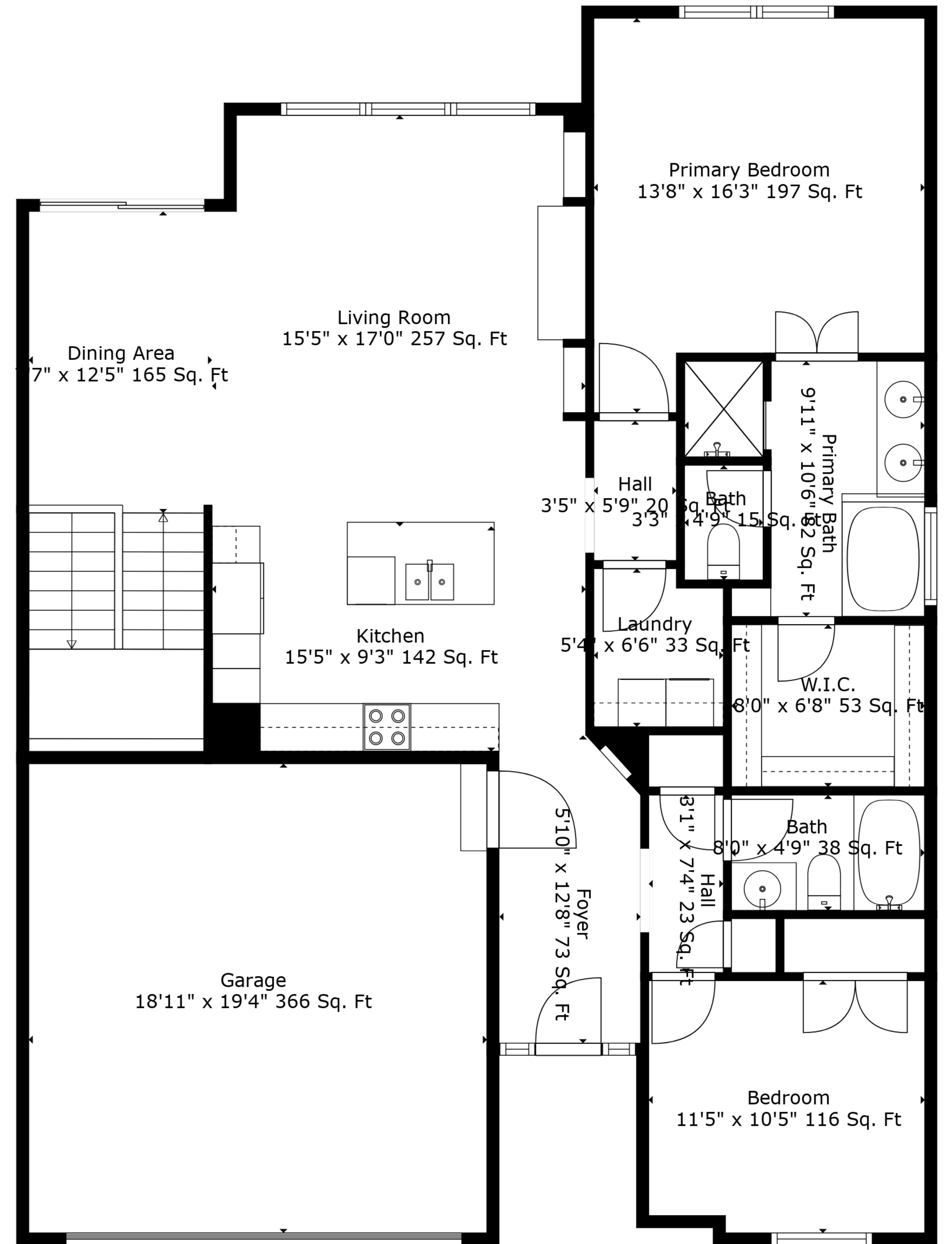
Floor 2
