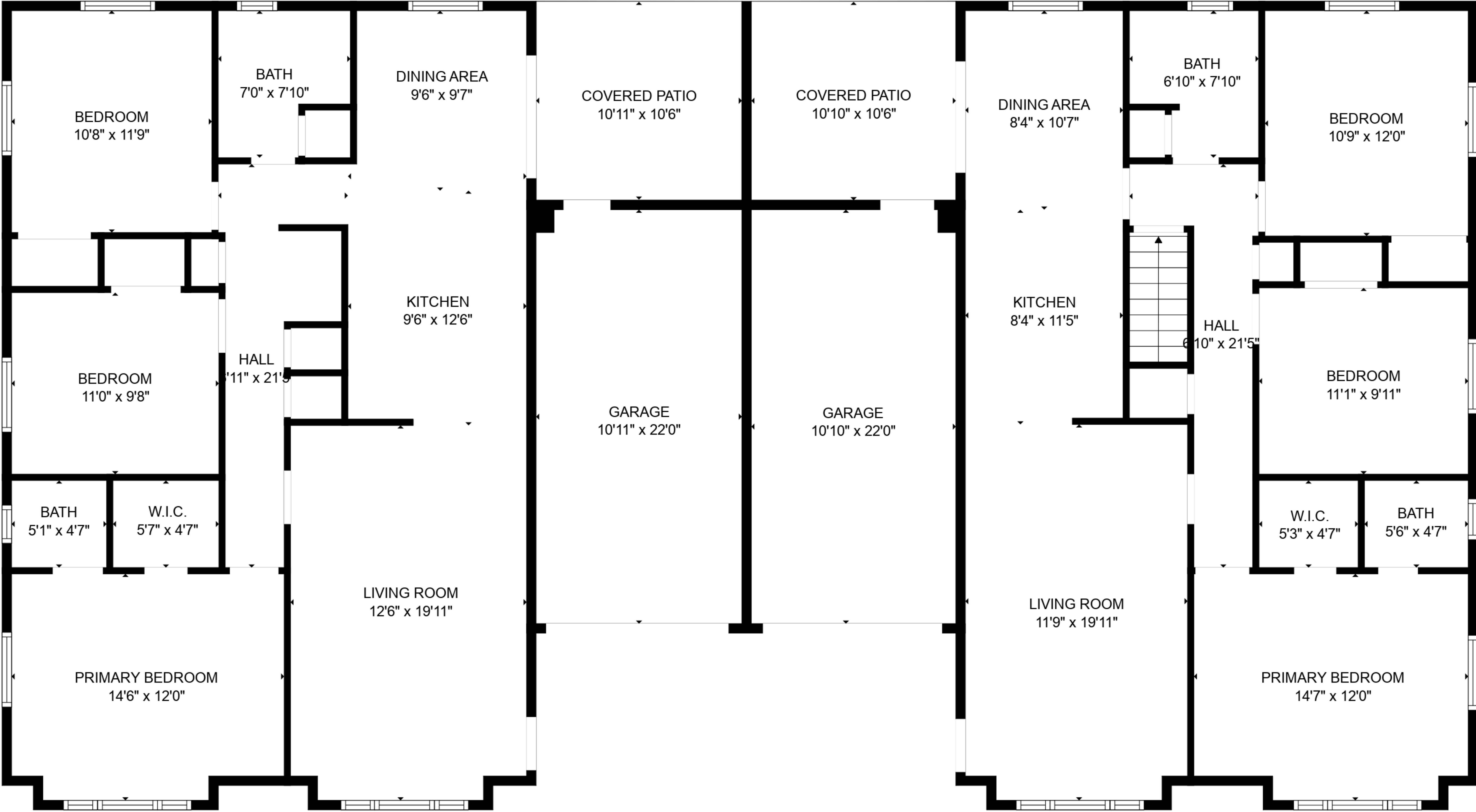
FLOOR 2
