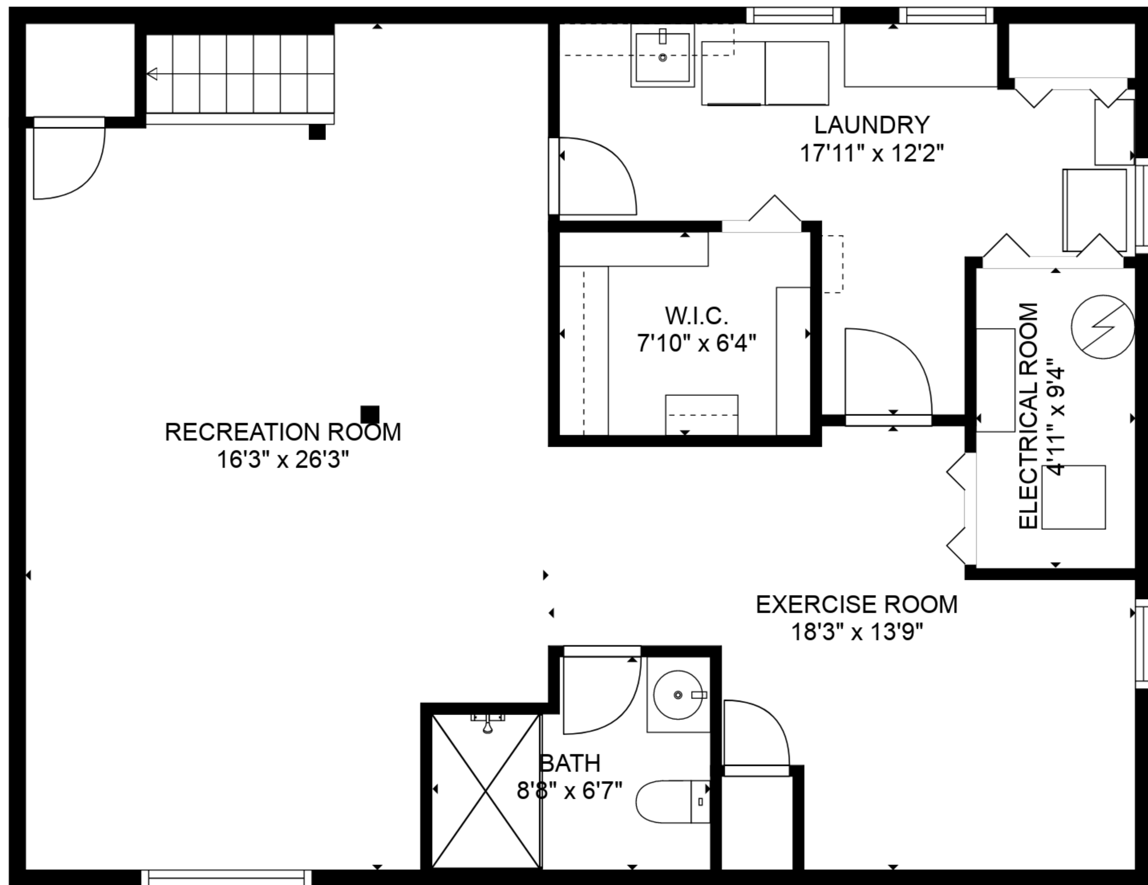
FLOOR 1
