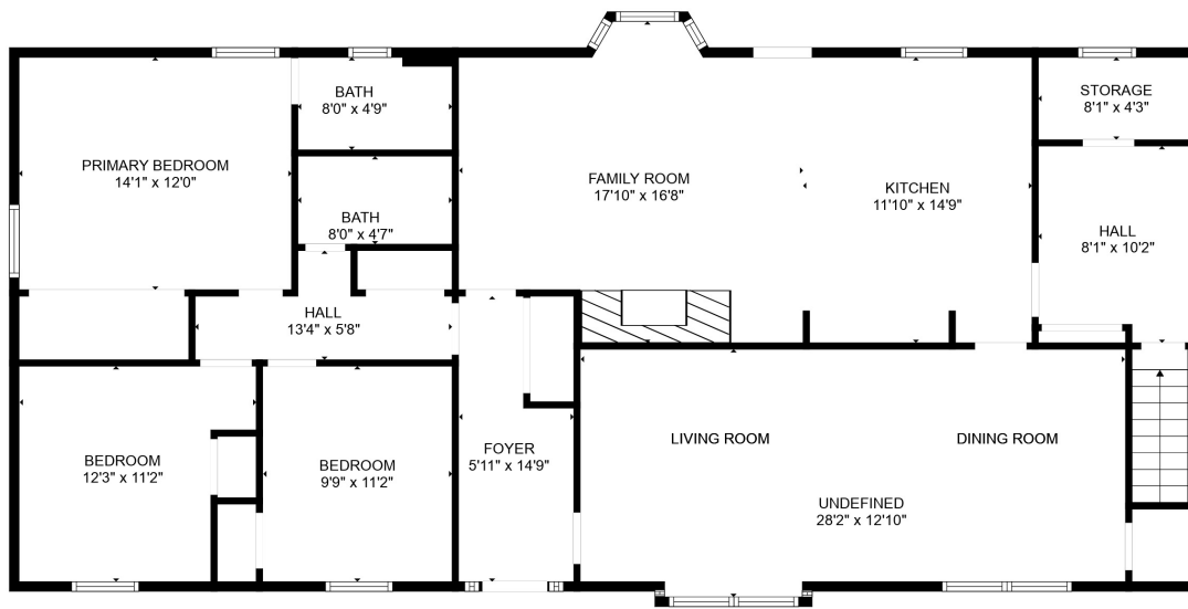
FLOOR 2
