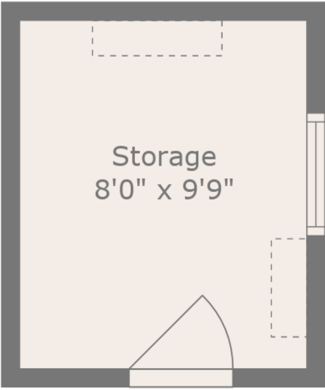
Floor 3
