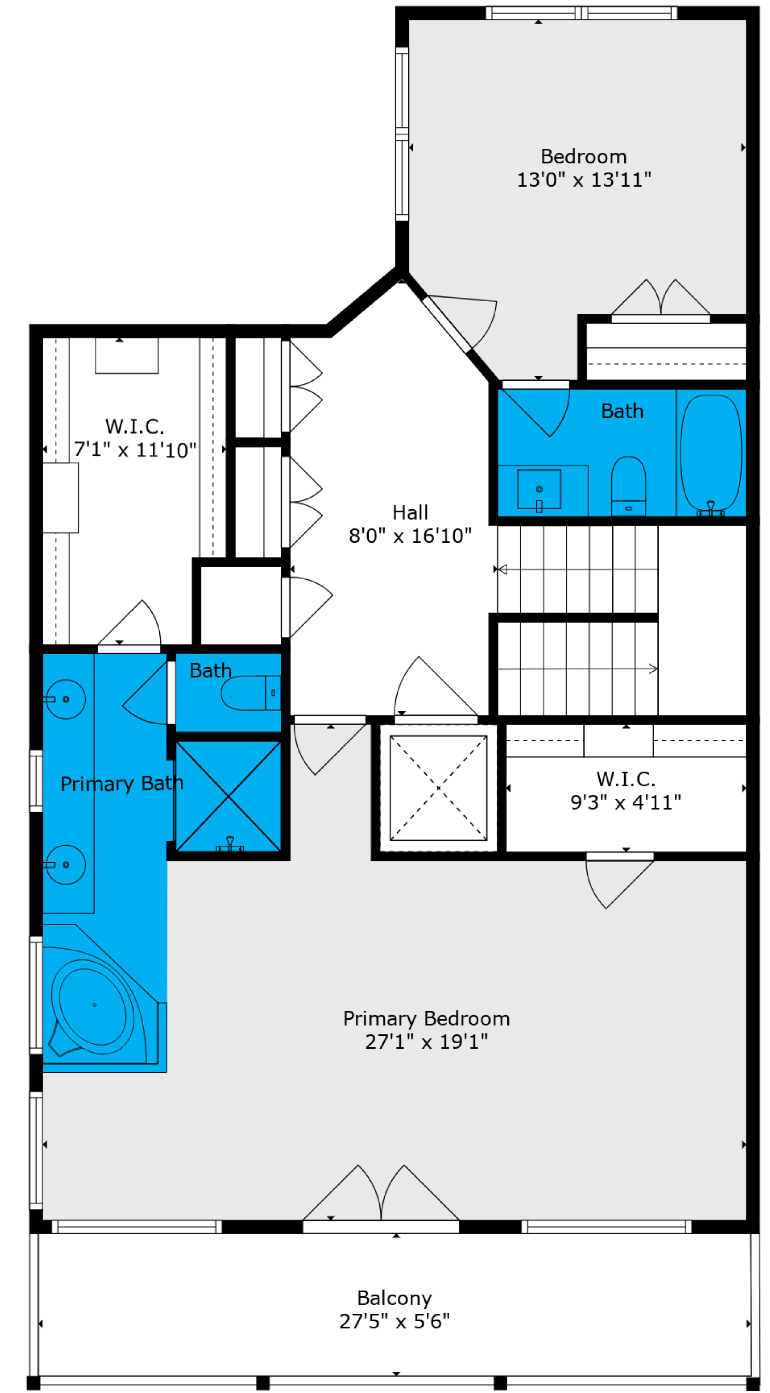
Floor 3
