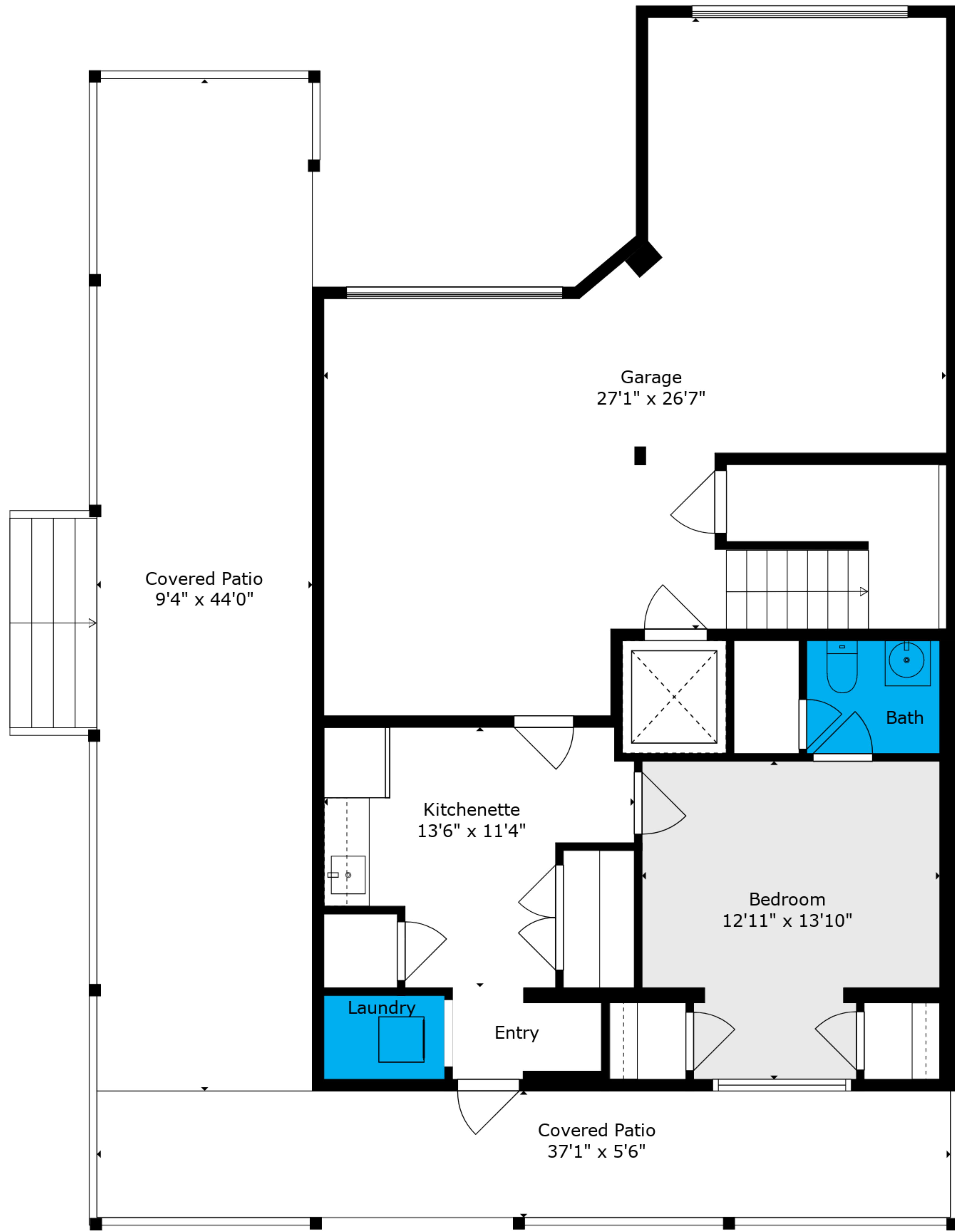
Floor 1
