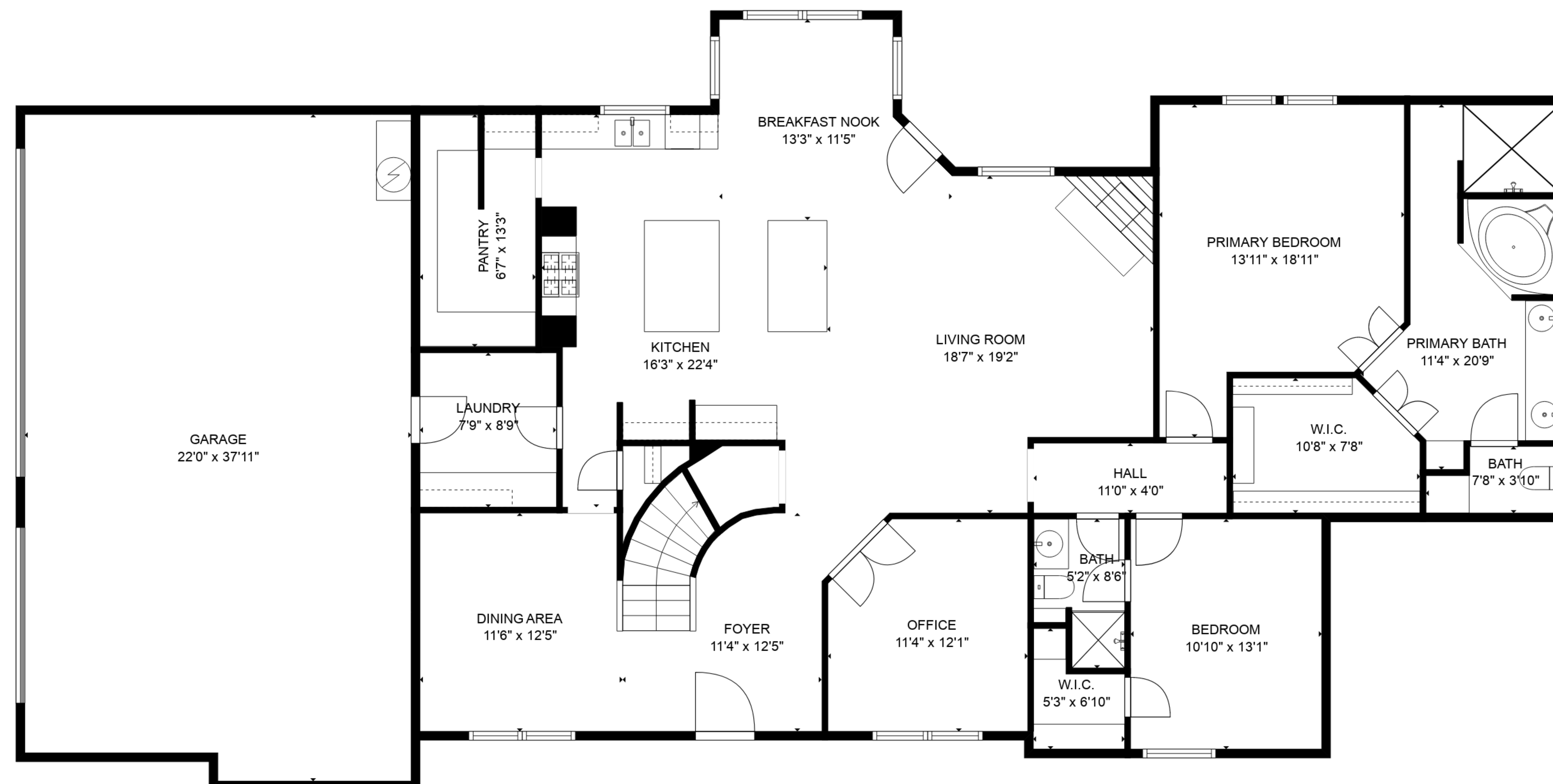
FLOOR 1
