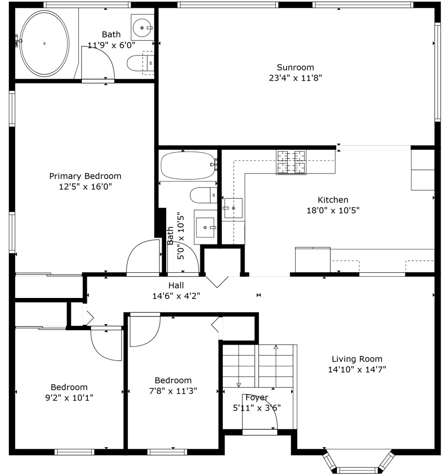
Floor 2
